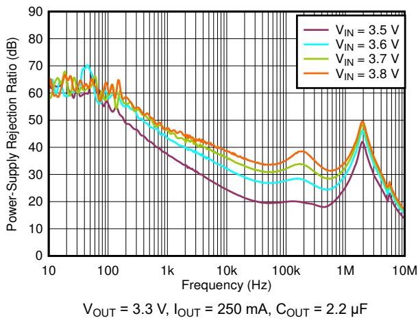
图 6-33. PSRR vs Frequency and V_{IN}
