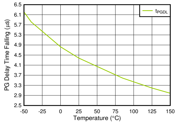
图 6-20. t_{PGDL} vs Temperature
