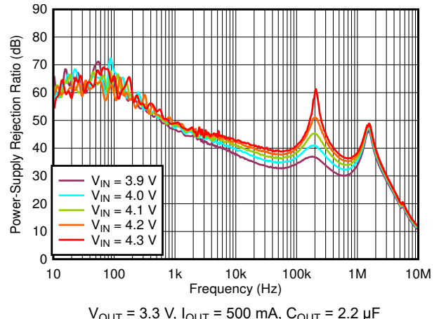
图 6-32. PSRR vs Frequency and V_{IN}
