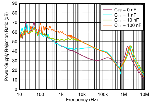
图 6-38. PSRR vs Frequency and C_{FF}
