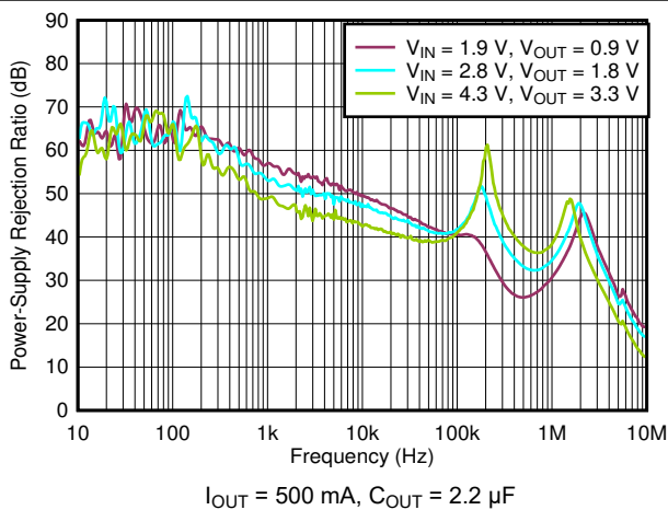
图 6-35. PSRR vs Frequency
