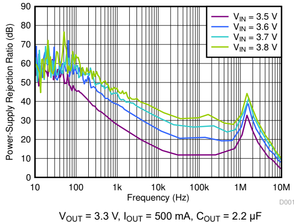
图 6-31. PSRR vs Frequency and V_{IN}
