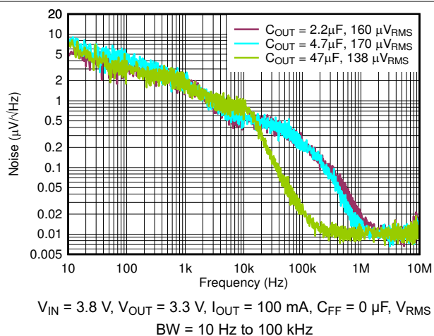
图 6-43. Output Spectral Noise Density vs Frequency and C_{OUT}
