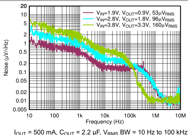
图 6-44. Output Spectral Noise Density vs Frequency
