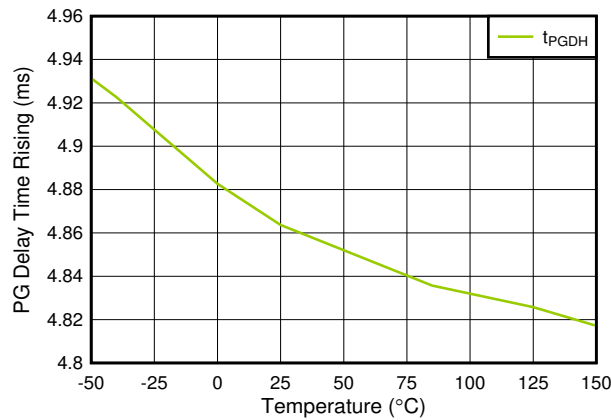
图 6-19. t_{PGDH} vs Temperature (For TPS746B Only)
