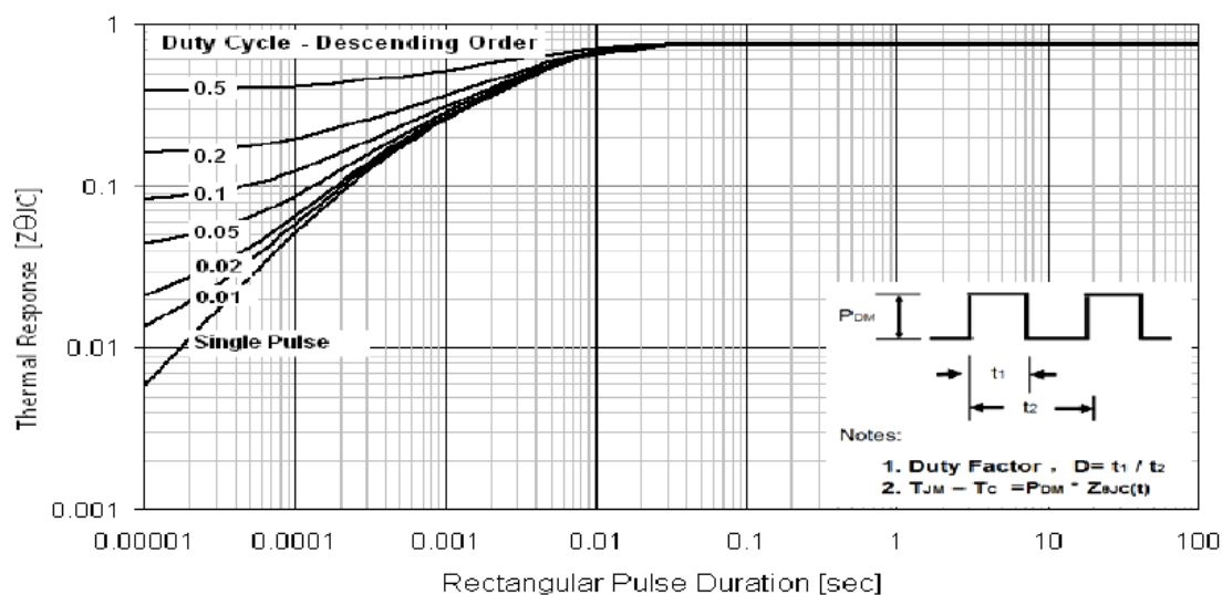
Transient Thermal Response Curve For JCS4N65RE/VE
