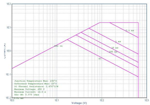
Maximum Safe Operating Area For JCS4N65RE/VE
