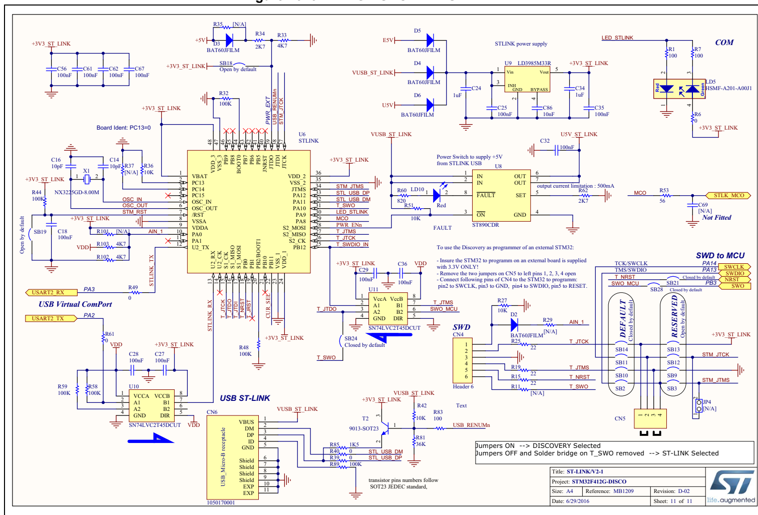
Figure 23. 32F412GDISCOVERY ST-LINK/V2-1
