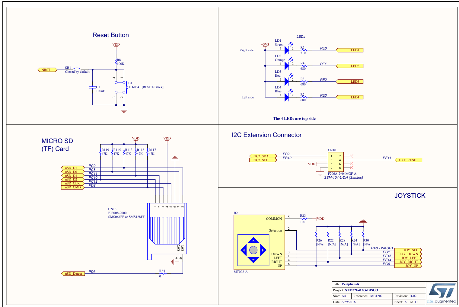
Figure 19. 32F412GDISCOVERY Peripherals
