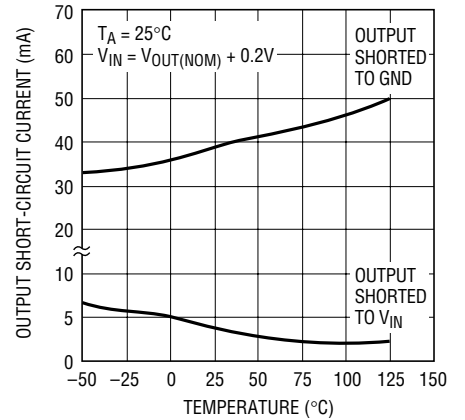
LTC1258 Series Output Short-Circuit Current vs Temperature
