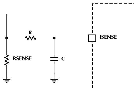
Figure 1. Current Limit with R_{SENSE}
