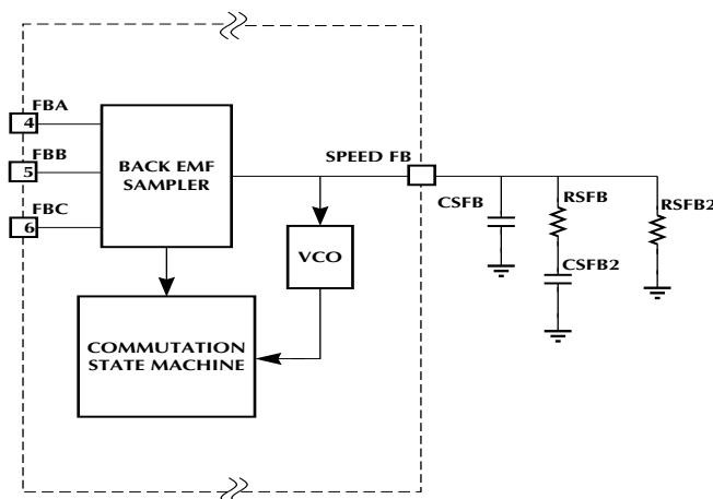
Figure 10. Phase Locked Loop
