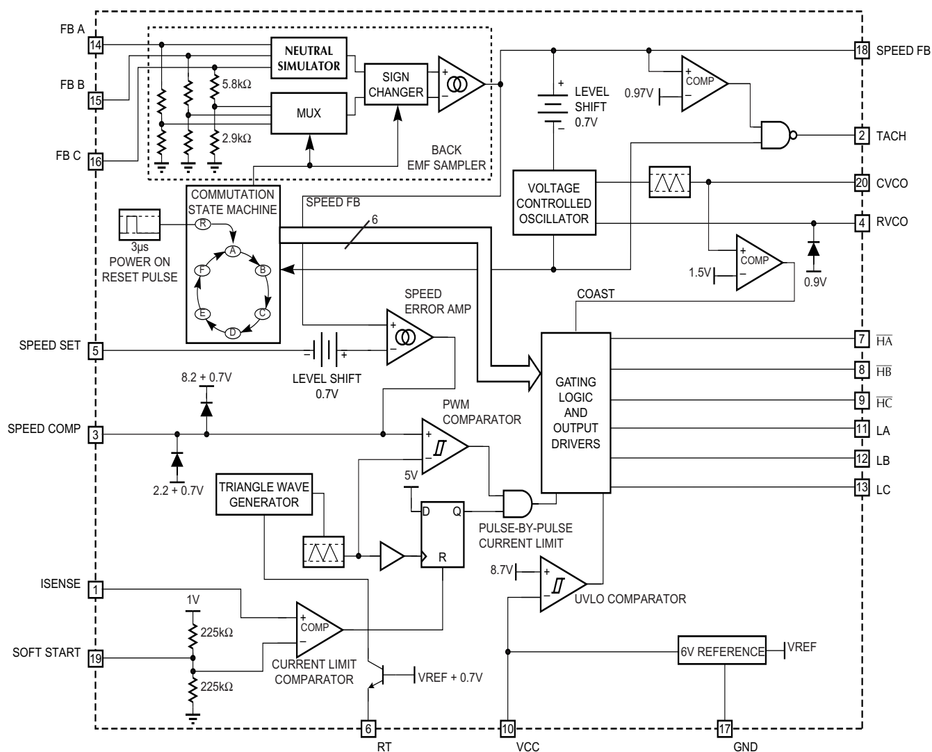
ML4435 Block Diagram
