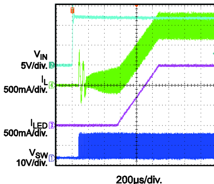
V_{IN} Start-Up
