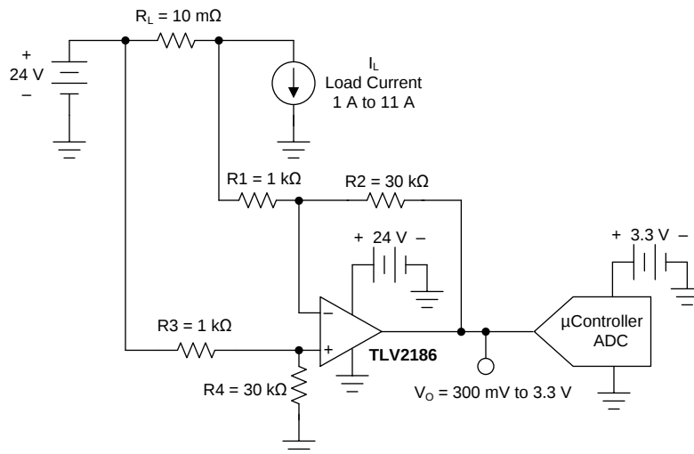
图 45. TLV2186 Configured as a High-Side Current Monitor
