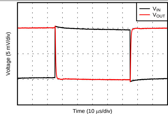
图 28. Negative Overload Recovery
