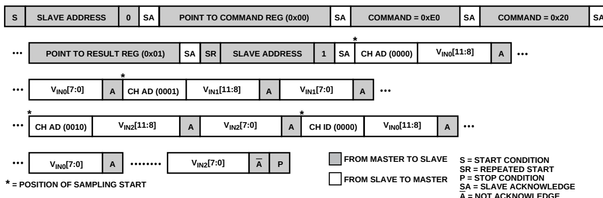
Figure 28. Command Mode Operation
