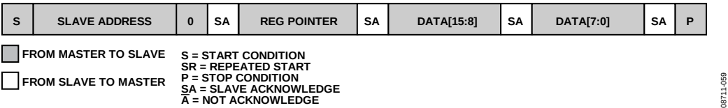
Figure 25. Writing Two Bytes of Data to a 16-Bit Register
