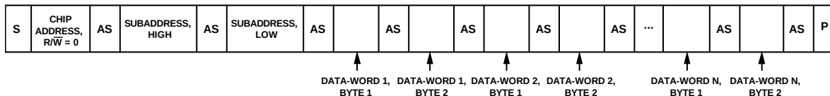
Figure 29. Simplified Burst Mode I 2 C Write Sequence
