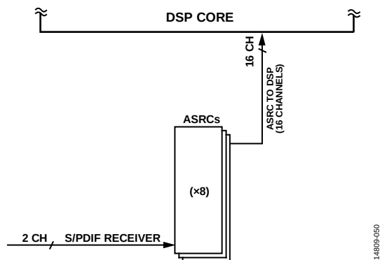
Figure 56. Example ASRC Routing for Asynchronous Input to the DSP Core
