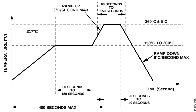
Figure 91. Soldering Profile
