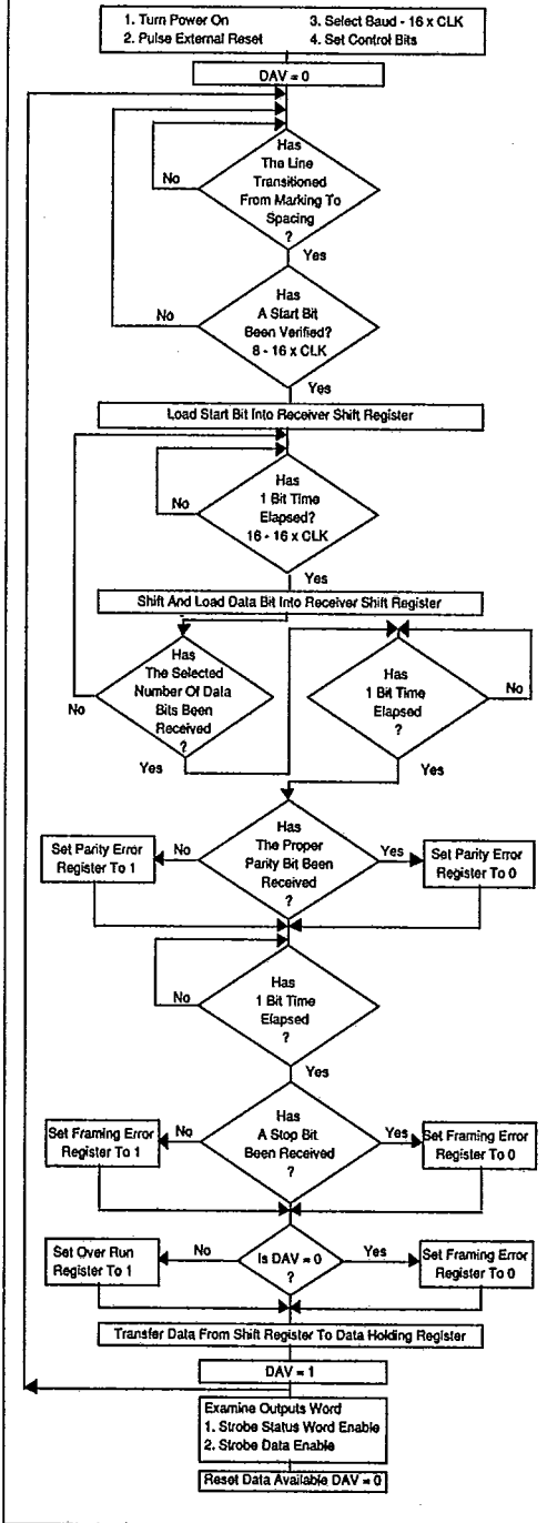
FIG. 23 RECEIVER OPERATION
