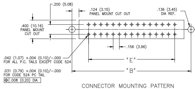
CONNECTOR MOUNTING PATTERN
