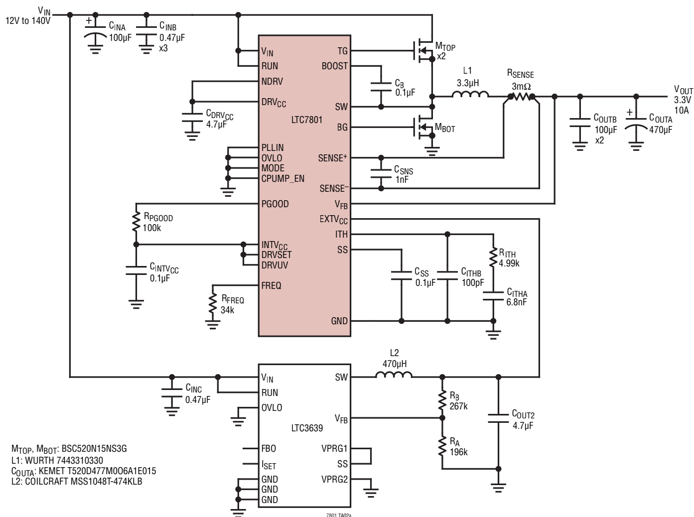
High Efficiency 140V to 3.3V Step-Down Regulator
