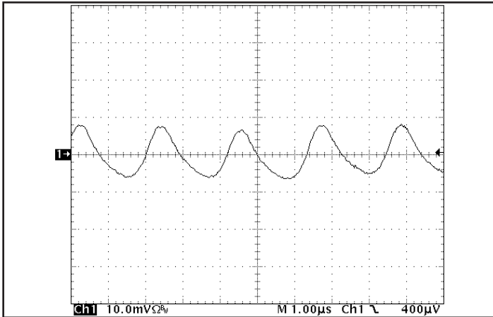
Figure 13: Input Terminal Ripple Current, i_c , at full rated output current and nominal input voltage with 10 \mu H source impedance and 47 \mu F electrolytic capacitor (200 mA/div). See Figure 12.
