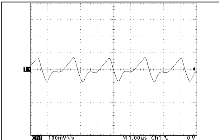
Figure 15: Output voltage ripple at nominal input voltage and rated load current (100 mV/div). Load capacitance: 1 \mu F ceramic capacitor and 15 \mu F tantalum capacitor. Bandwidth: 20 Mhz. See Figure 12.
