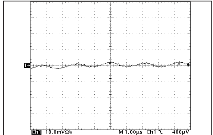
Figure 14: Input reflected ripple current, i_s , through a 10 \mu H source inductor at nominal input voltage and rated load current (10 mA/div). See Figure 12.
