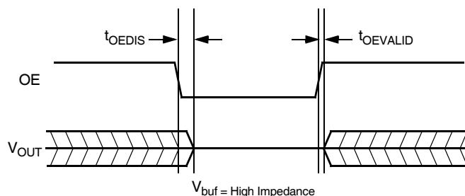
V_{buf} OUTPUT ENABLE TIMING
