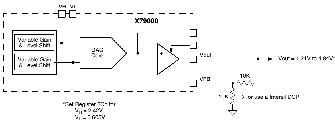
FIGURE 4. ACHIEVING HIGHER OUTPUT VOLTAGES
