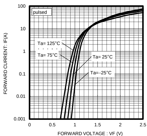
Fig.1 VF-IF Characteristics
