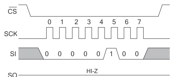
Figure 9. WRDI Instruction
