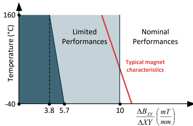
Figure 7 - Minimum useful signal definition for rotary stray-field immune application-low field variant
