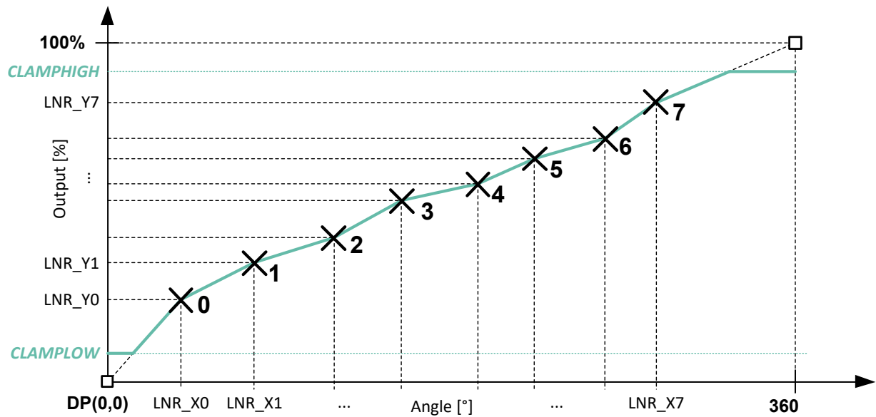
Figure 18 – 8-pts Linearization Parameters Description
