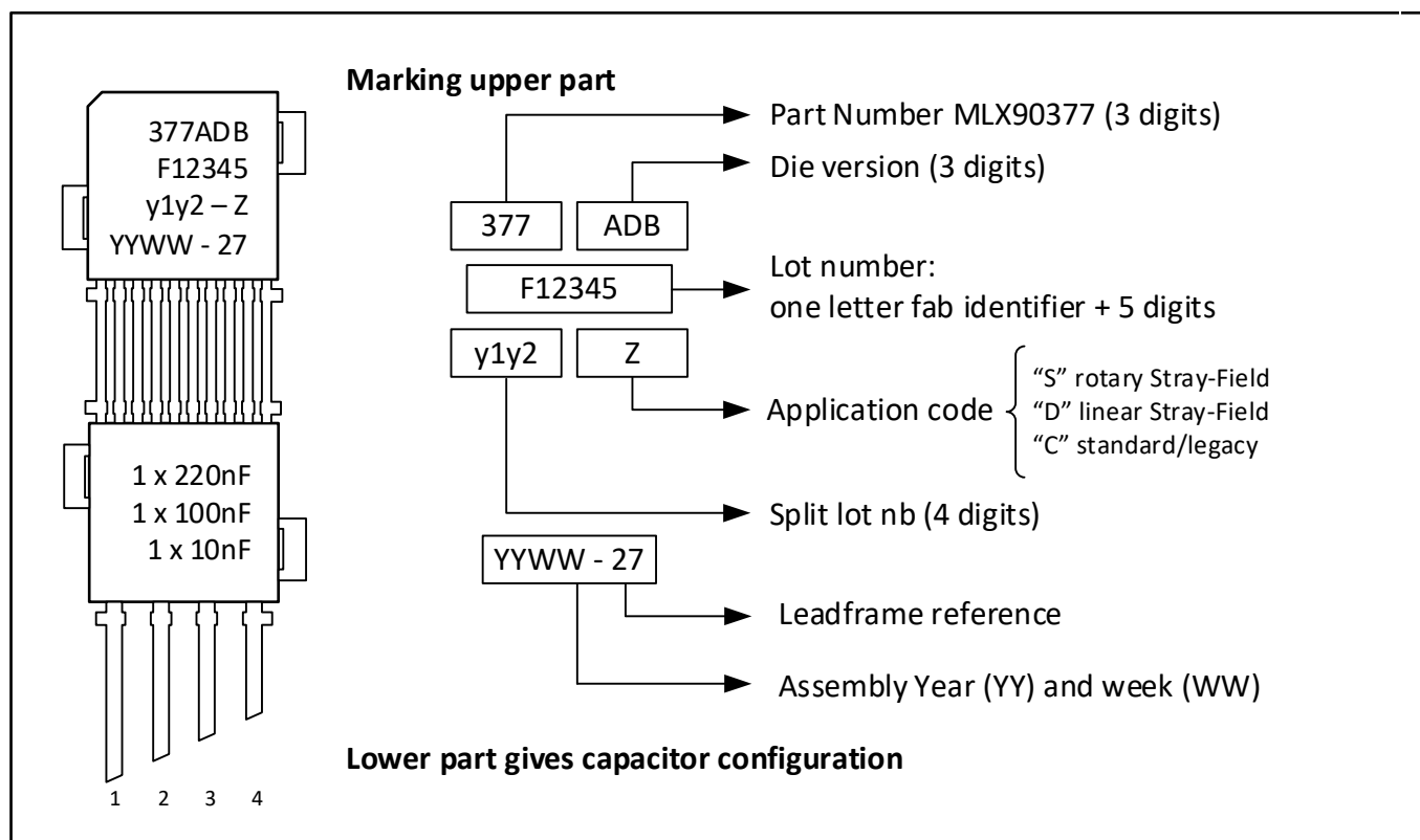
Figure 39 - DMP-4 Marking
