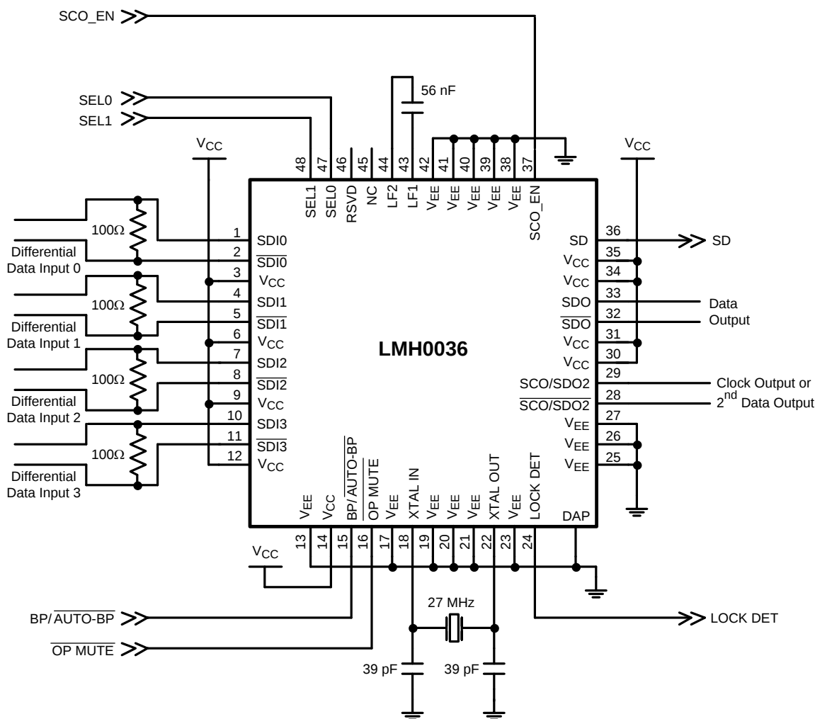
Figure 5 shows a application circuit for the LMH0036.
