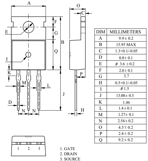
KHB7D0N65P1
