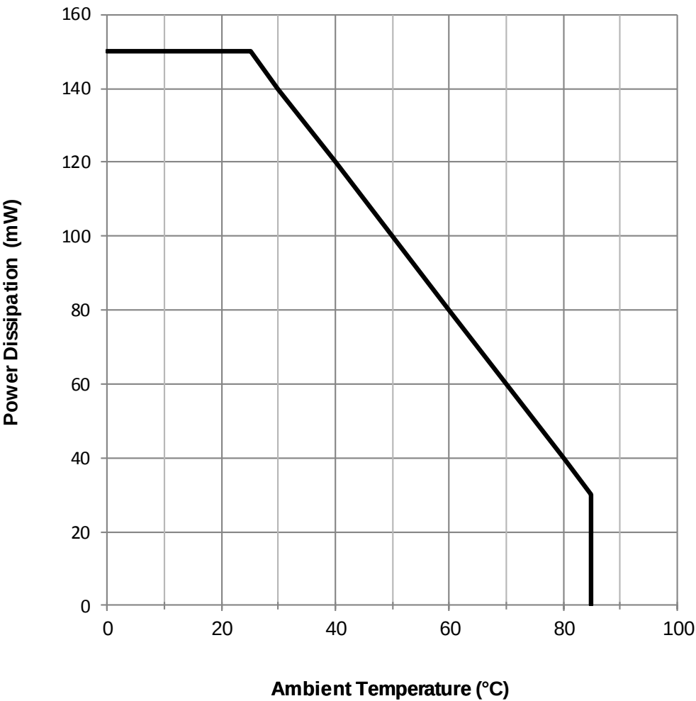
Derating Curve:
