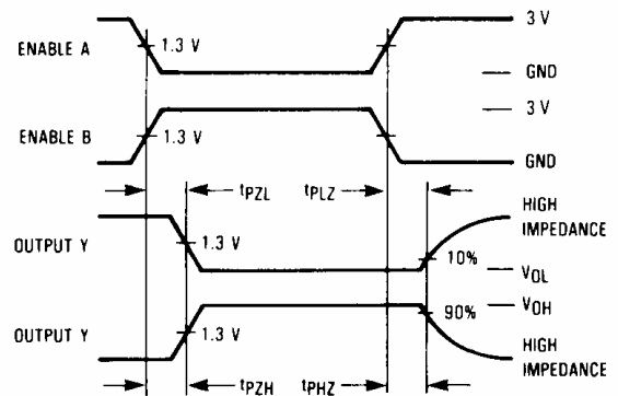
Figure 2. Switching Waveforms
