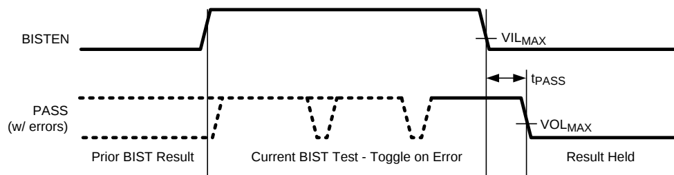
Figure 12. BIST PASS Waveform
