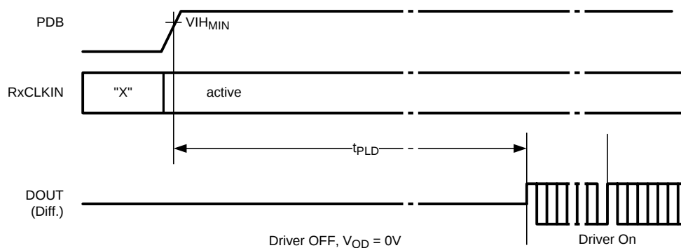
Figure 7. Lock Time
