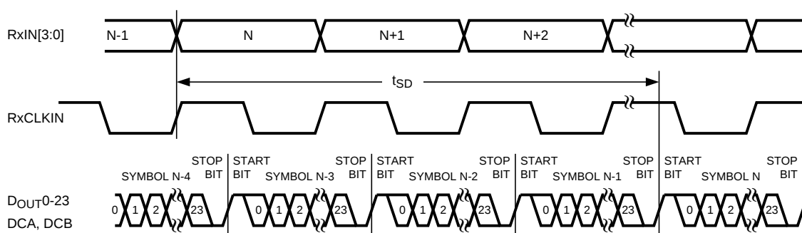
Figure 9. Latency Delay
