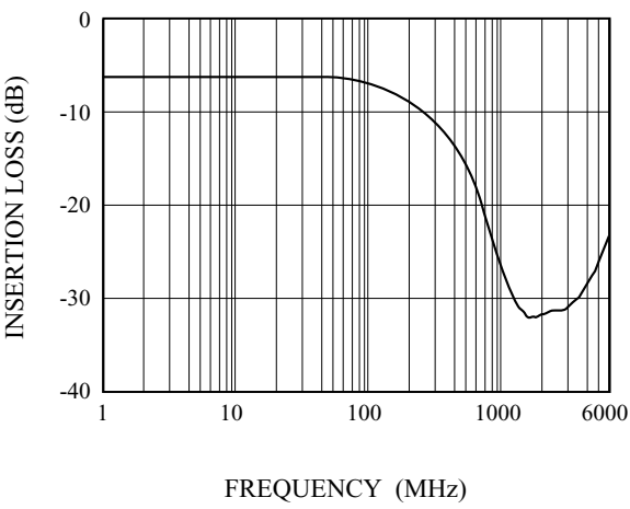
S_{21} - F
