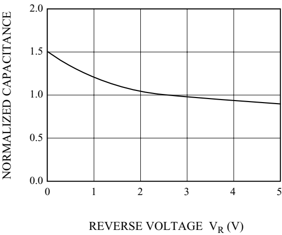
C_J - V_R
