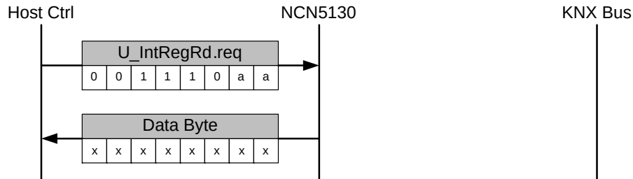
Figure 43. Internal Register Read Service
