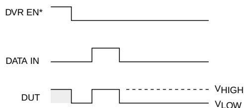
Figure 2. Driver Functionality
