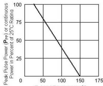
FIGURE 3 Derating Curve
