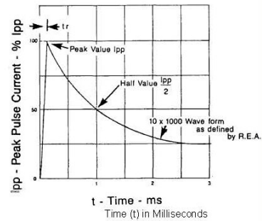
FIGURE 2 Pulse Waveform for Exponential Surge
