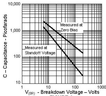
FIGURE 4 P5KE Typical Capacitance vs. Breakdown Voltage
