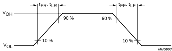
Fig 5. Rise and fall times.
