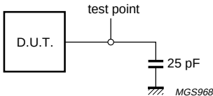
Fig 11. Load on pins VM/VMO, VP/VPO and RCV.
