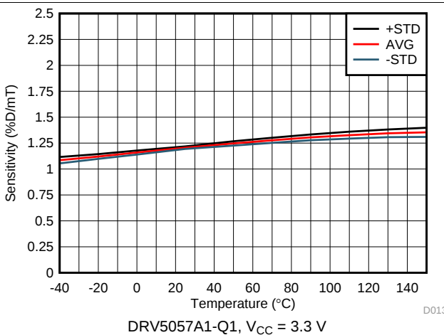
Figure 5. Sensitivity vs Temperature
