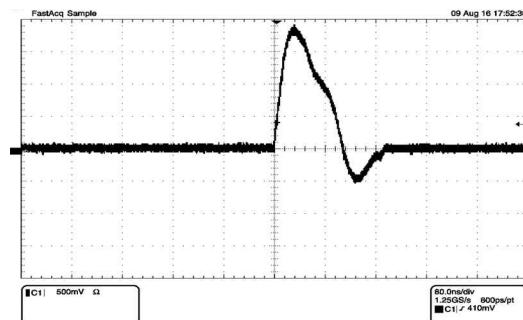
mV per Div 500 mV nS per Div 80 ns 图 7-19. 10BASE-Tc Link Pulse Waveform
