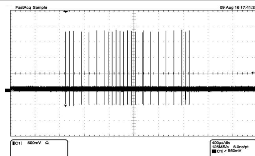
mV per Div 500 mV µ S per Div 400 µ s 图 7-21. Auto-Negotiation Fast Link Pulses Waveform
