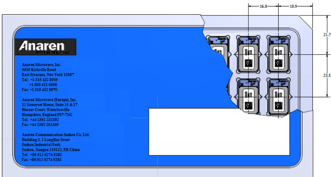
Figure 12 A2530E24A and A2530E24C Matrix Tray Packaging Detail (27/Tray)
