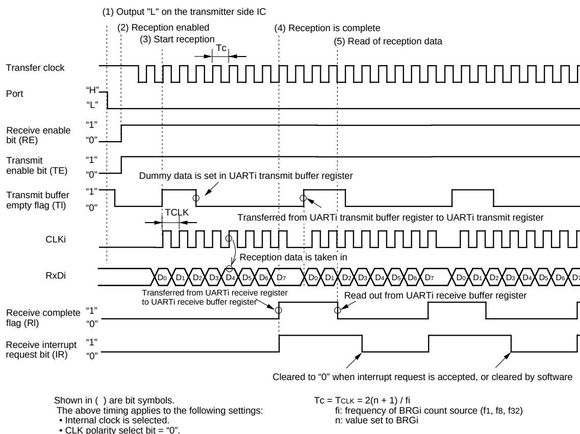
Figure 2.5.11. Operation timing of reception in serial interface special function master mode, with clock delay
