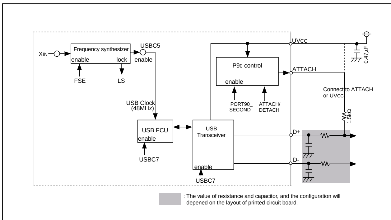
Figure 2.8.51. Peripheral circuit block diagram
