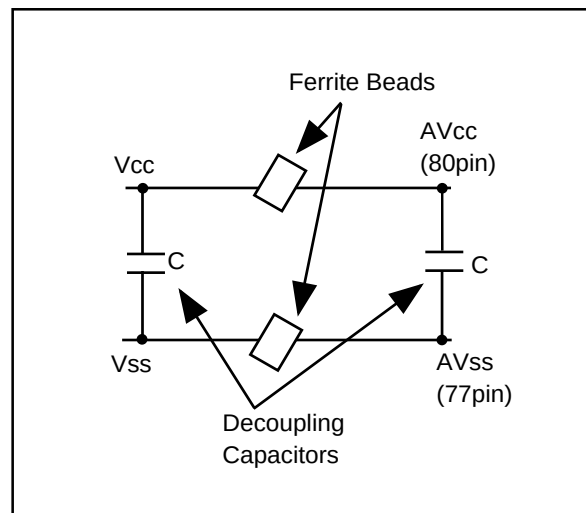
Figure 2.8.53. Decoupling capacitor
