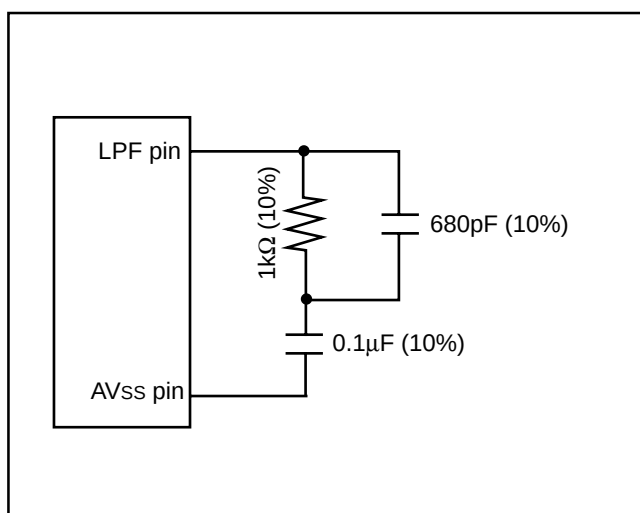
Figure 2.8.52. Passive part of LPF pin
