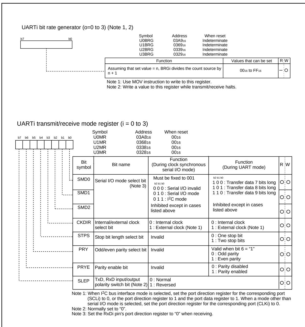
Figure 2.4.4. UARTi-related registers (2)
