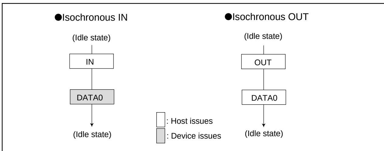
Figure 2.8.6. Isochronous transfer
