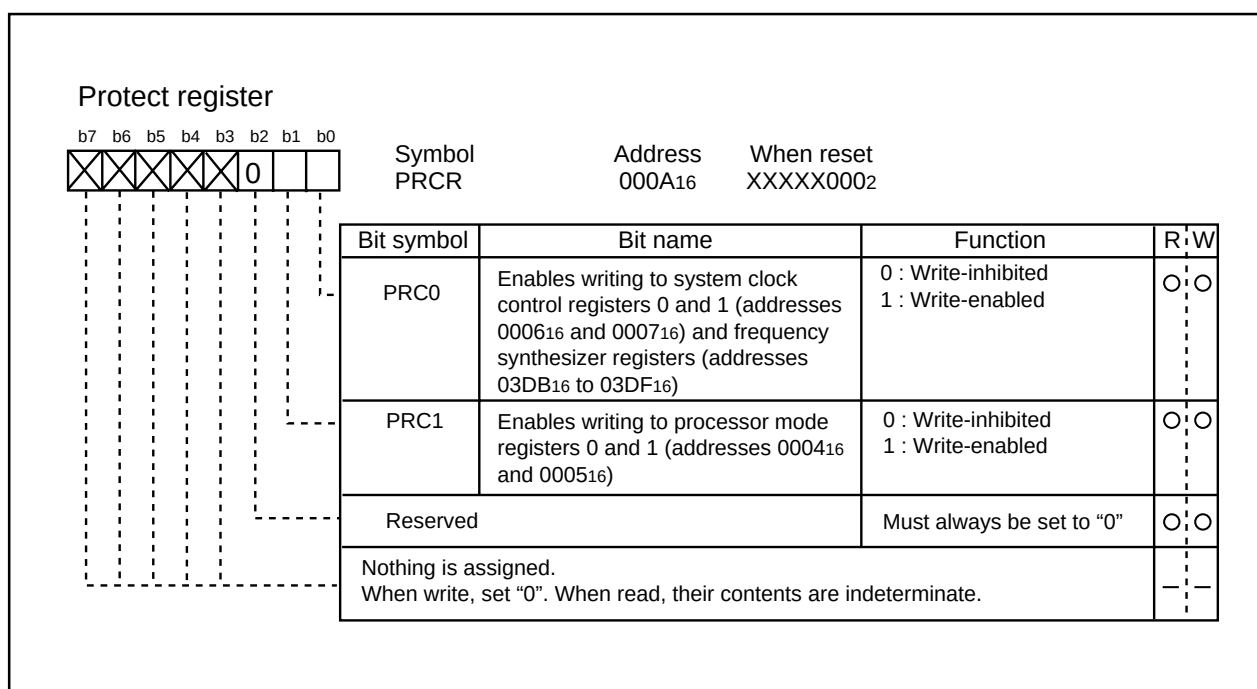
Figure 2.1.1. Protect register
