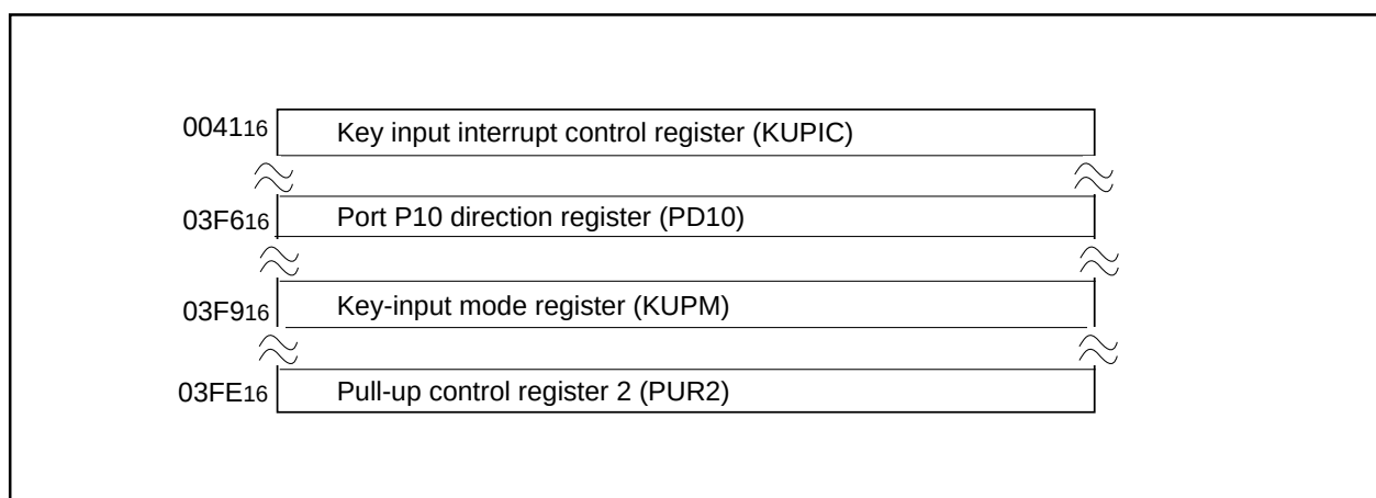
Figure 2.14.1. Memory map of key-input interrupt-related registers
