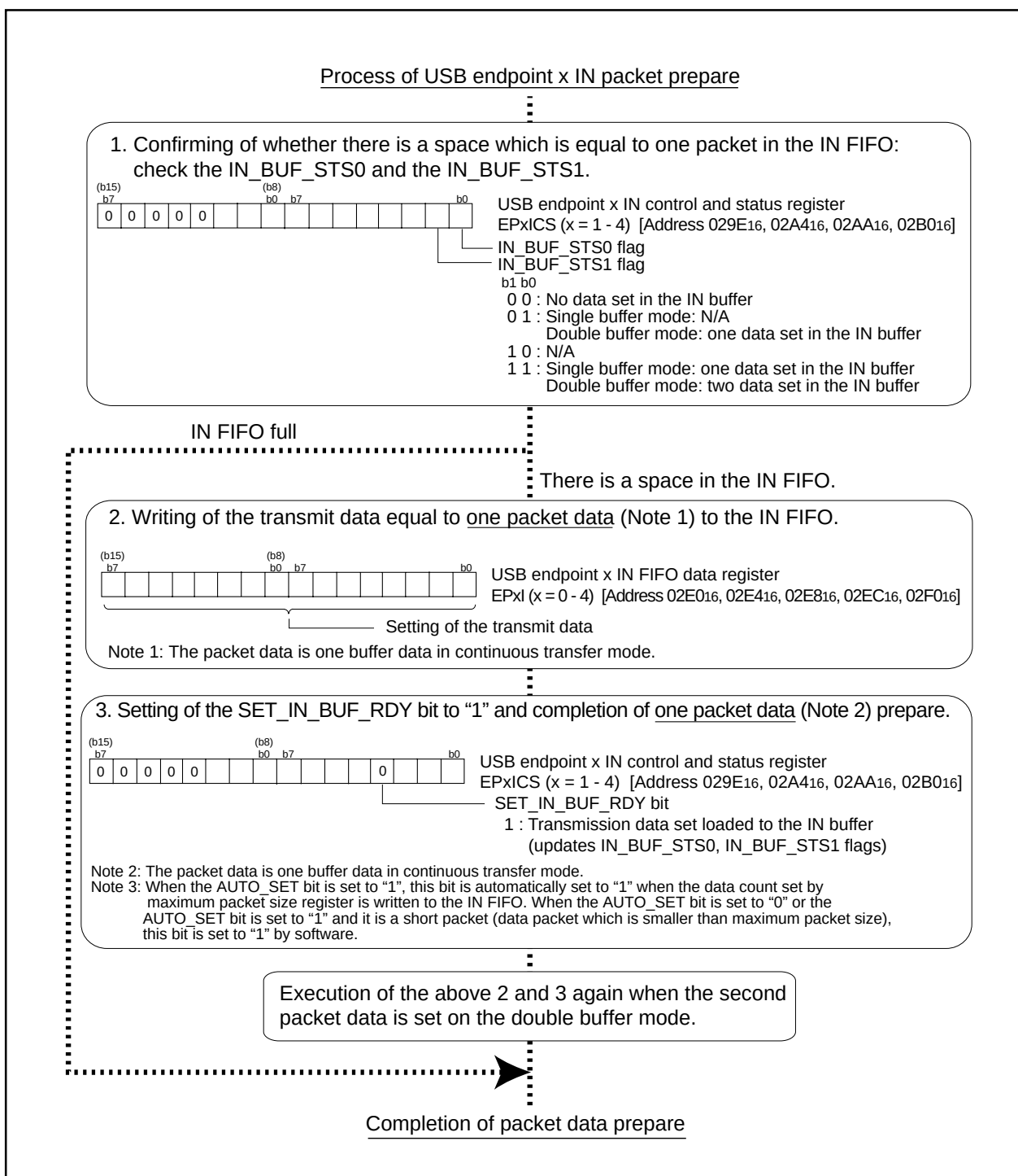
Figure 2.8.49. Endpoint 1 to 4 IN packet prepare routine
