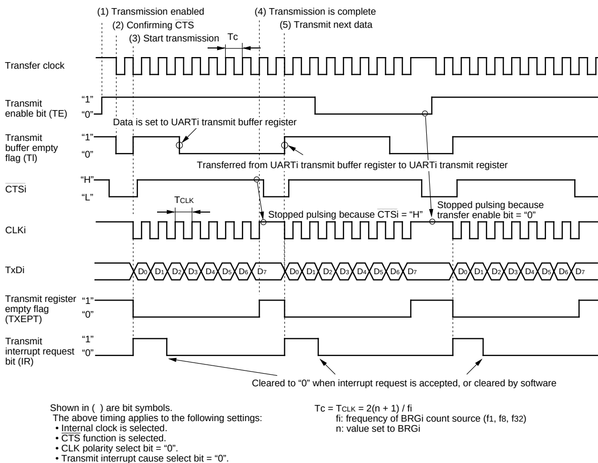
Figure 2.3.5. Operation timing of transmission in clock-synchronous serial I/O mode
