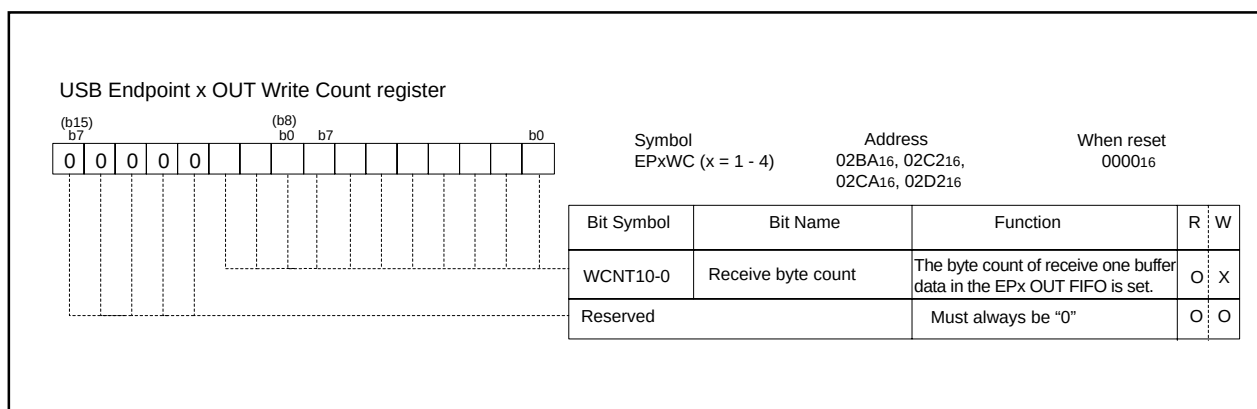
Figure 2.8.42. USB endpoint x(x=1 to 4) OUT write count register
