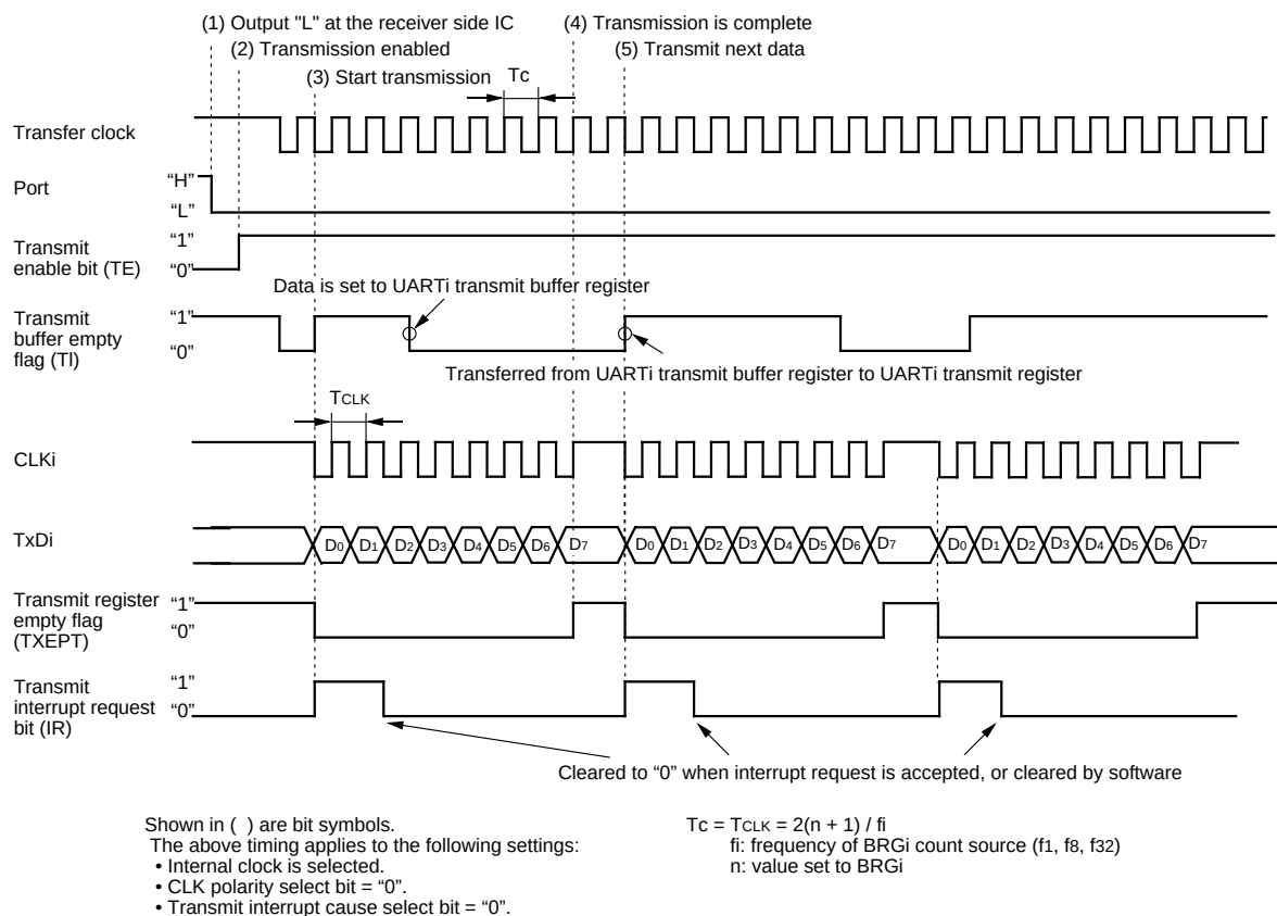
Figure 2.5.8. Operation timing of transmission in serial interface special function master mode, without clock delay
