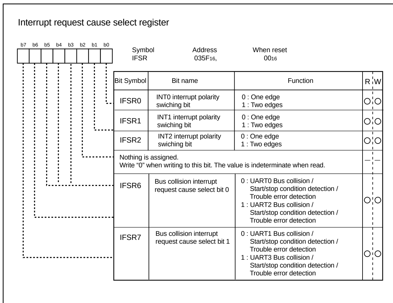
Figure 2.4.6. UARTi-related registers (4)
