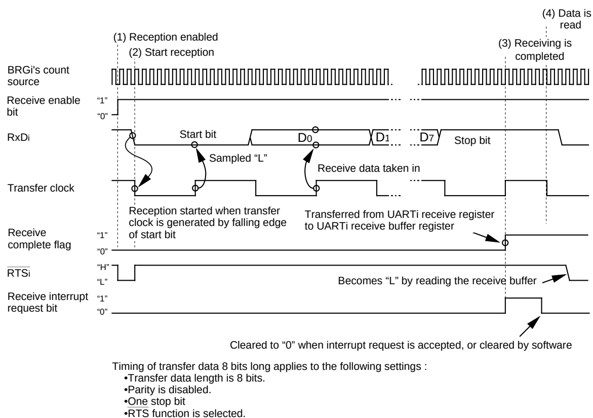
Figure 2.4.10. Operation timing of reception in UART mode
