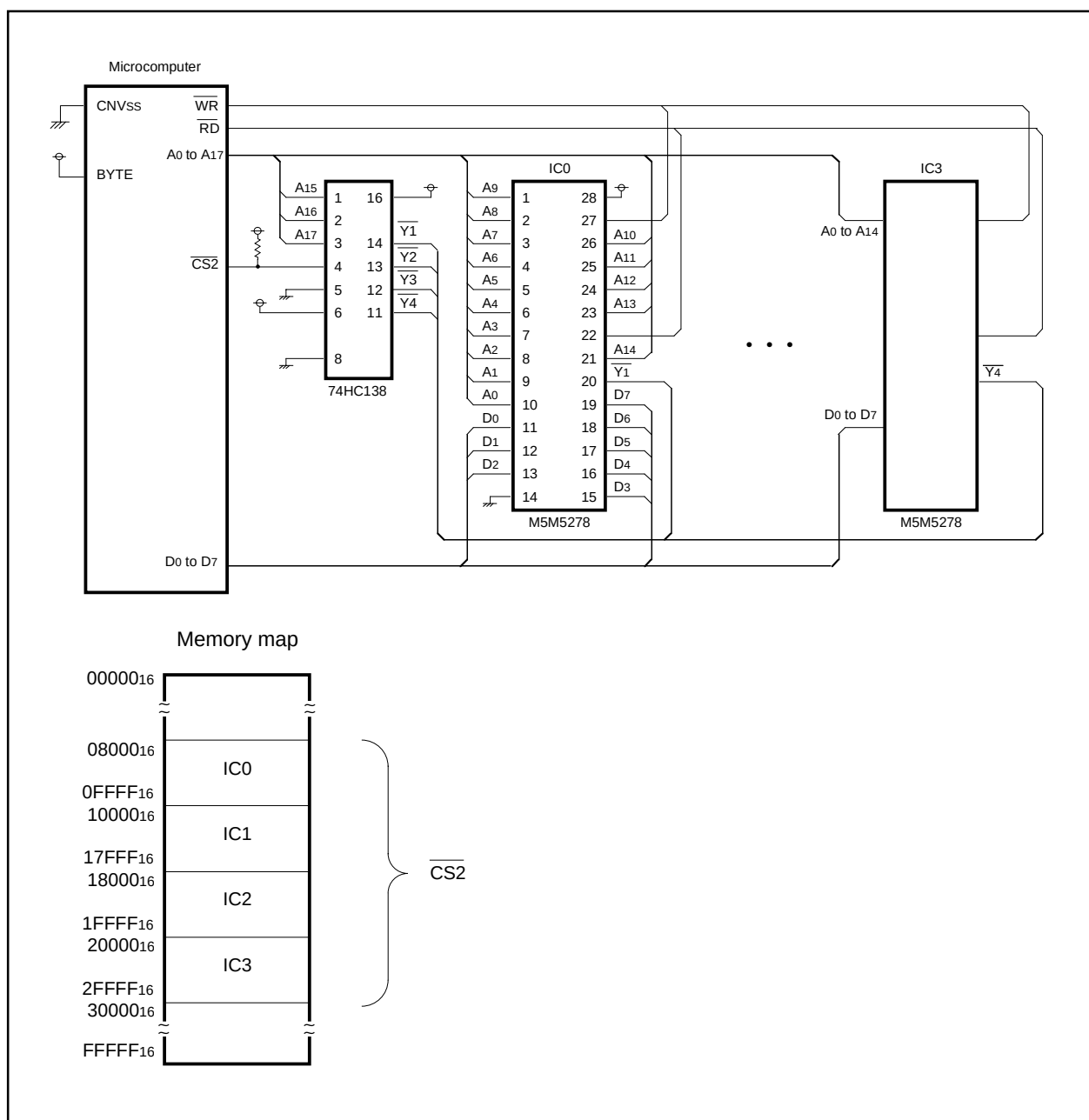
Figure 4.3.6. Chip selects and address bus
