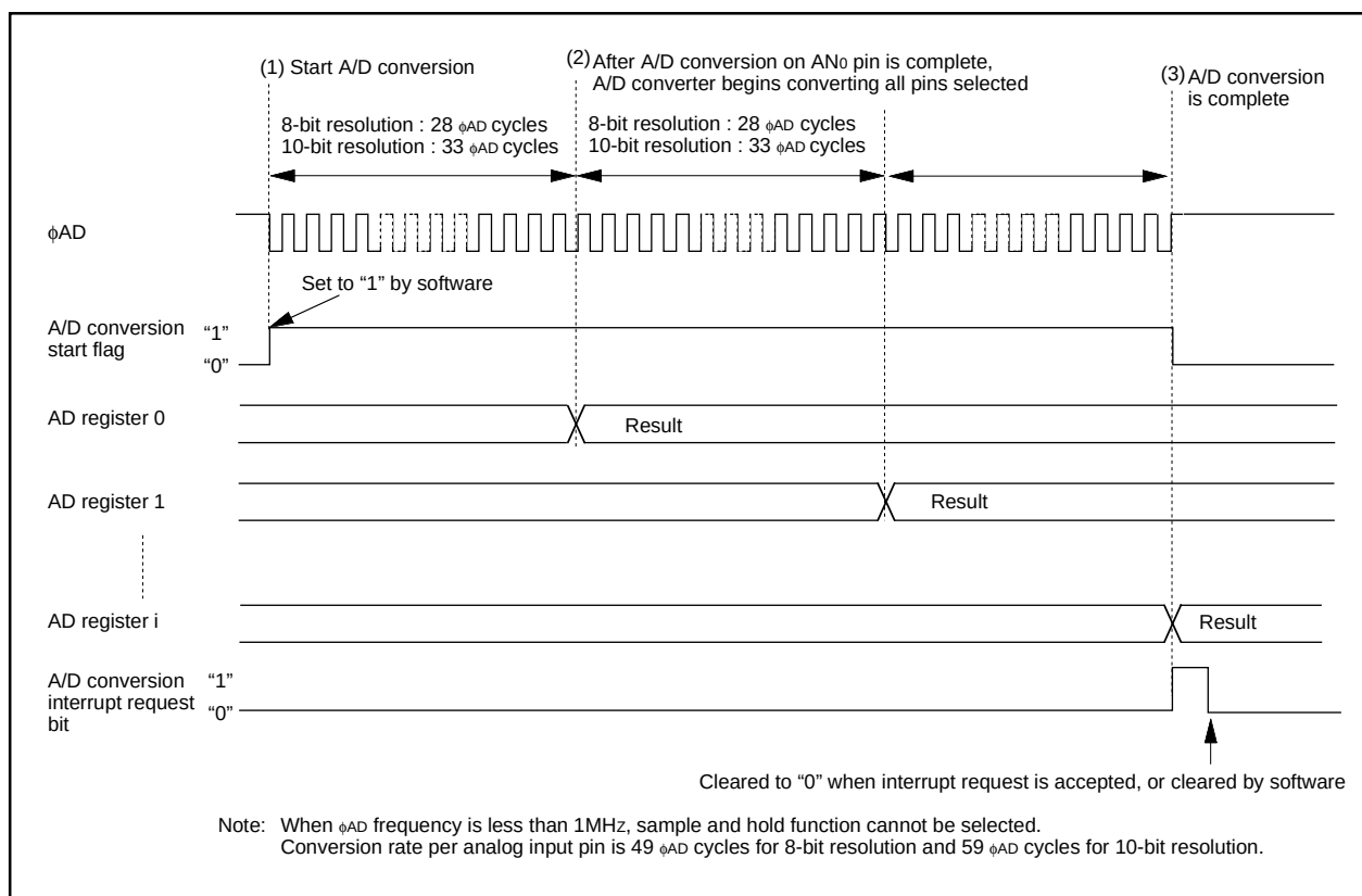
Figure 2.9.10. Operation timing of single sweep mode
