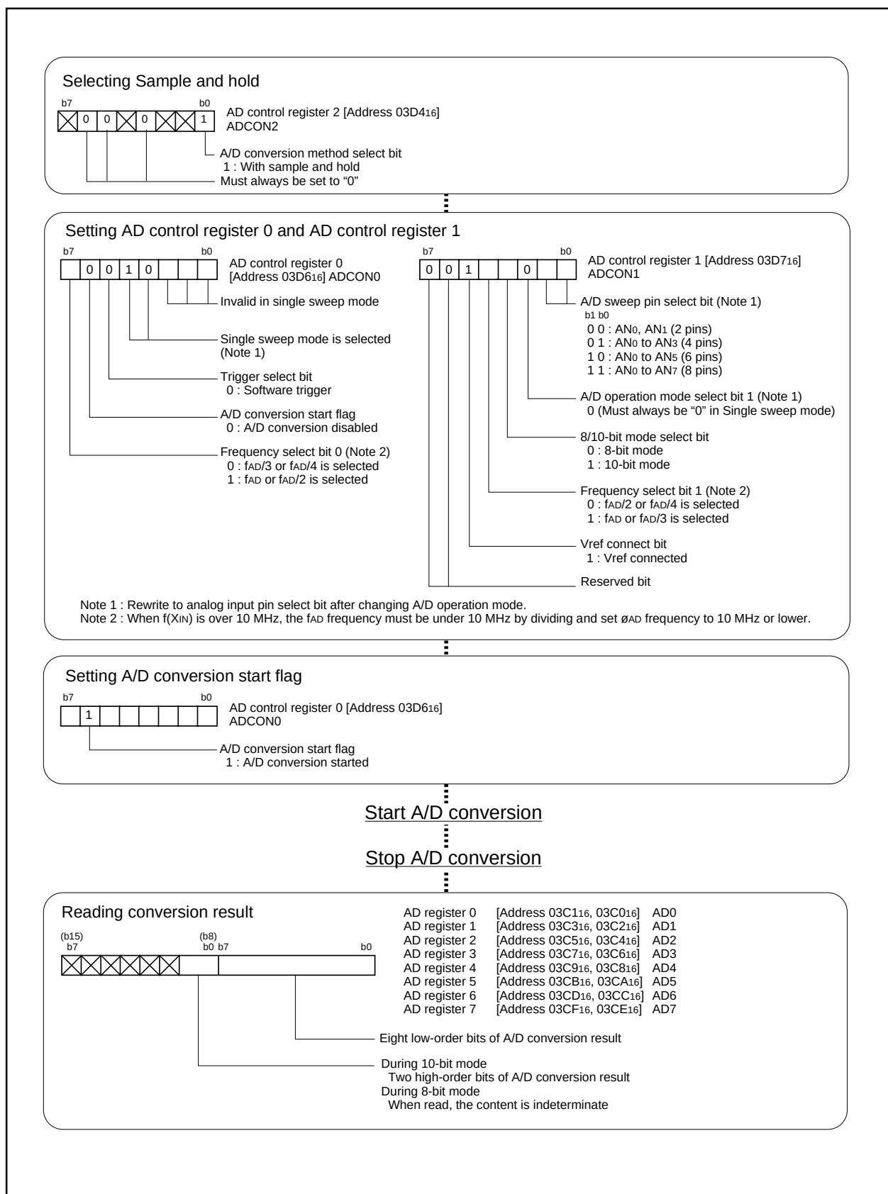
Figure 2.9.11. Set-up procedure of single sweep mode
