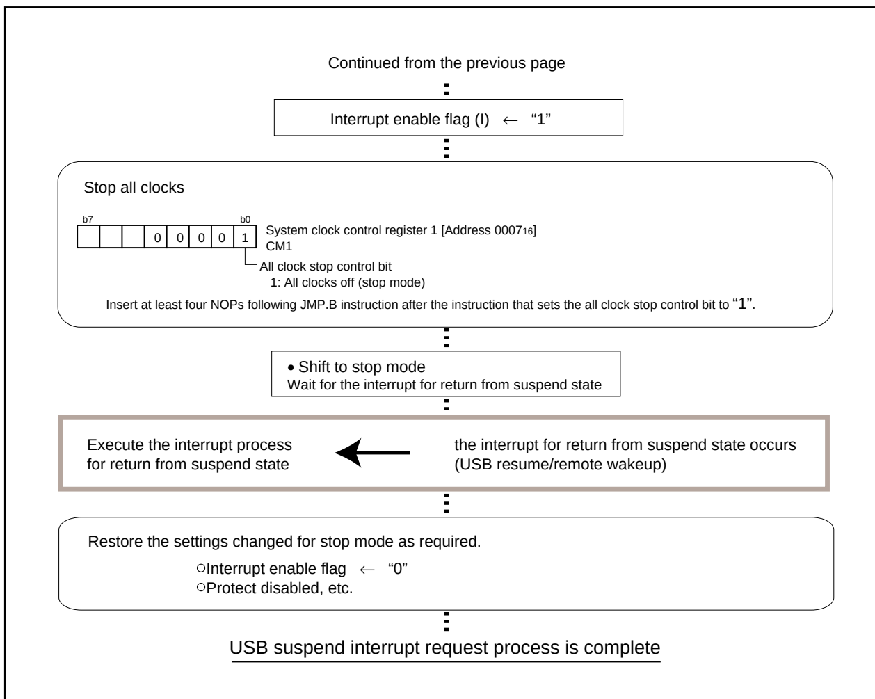
Figure 2.8.29. USB suspend interrupt request processing routine (2)
