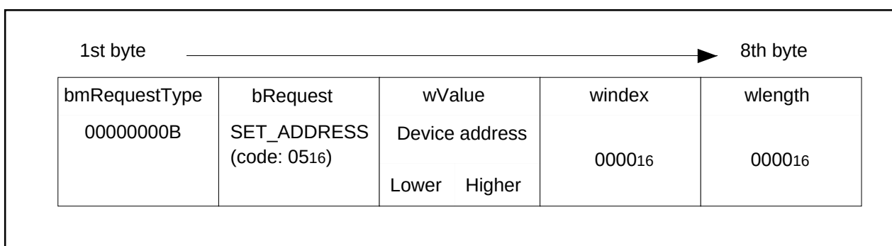
Figure 2.8.35. SET_ADDRESS Request
