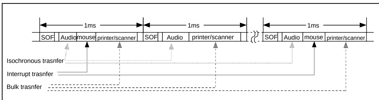
Figure 2.8.1. Frame image
