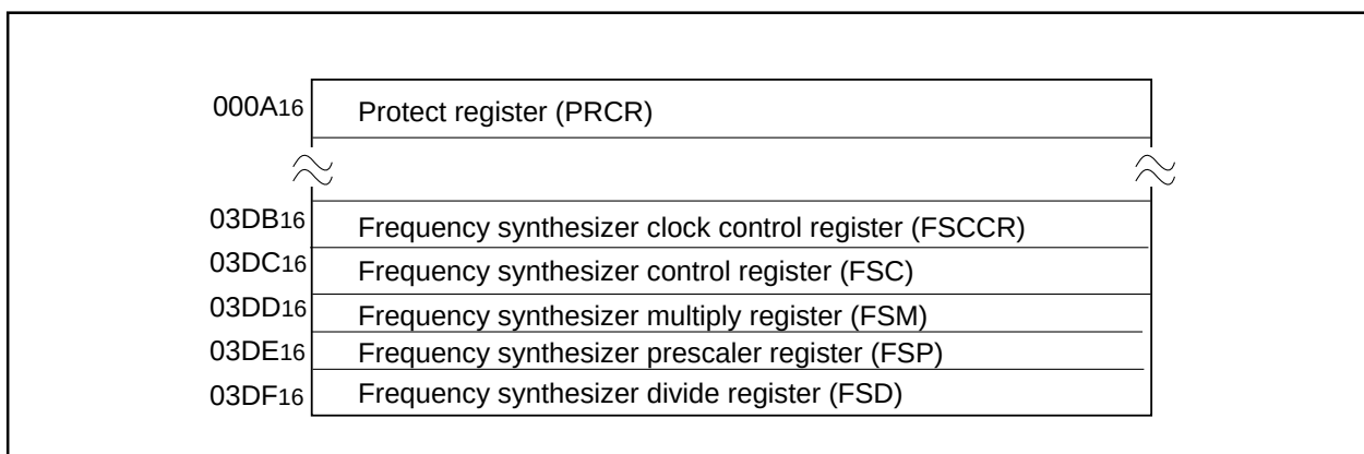
Figure 2.7.2. Memory map of frequency synthesizer related registers
