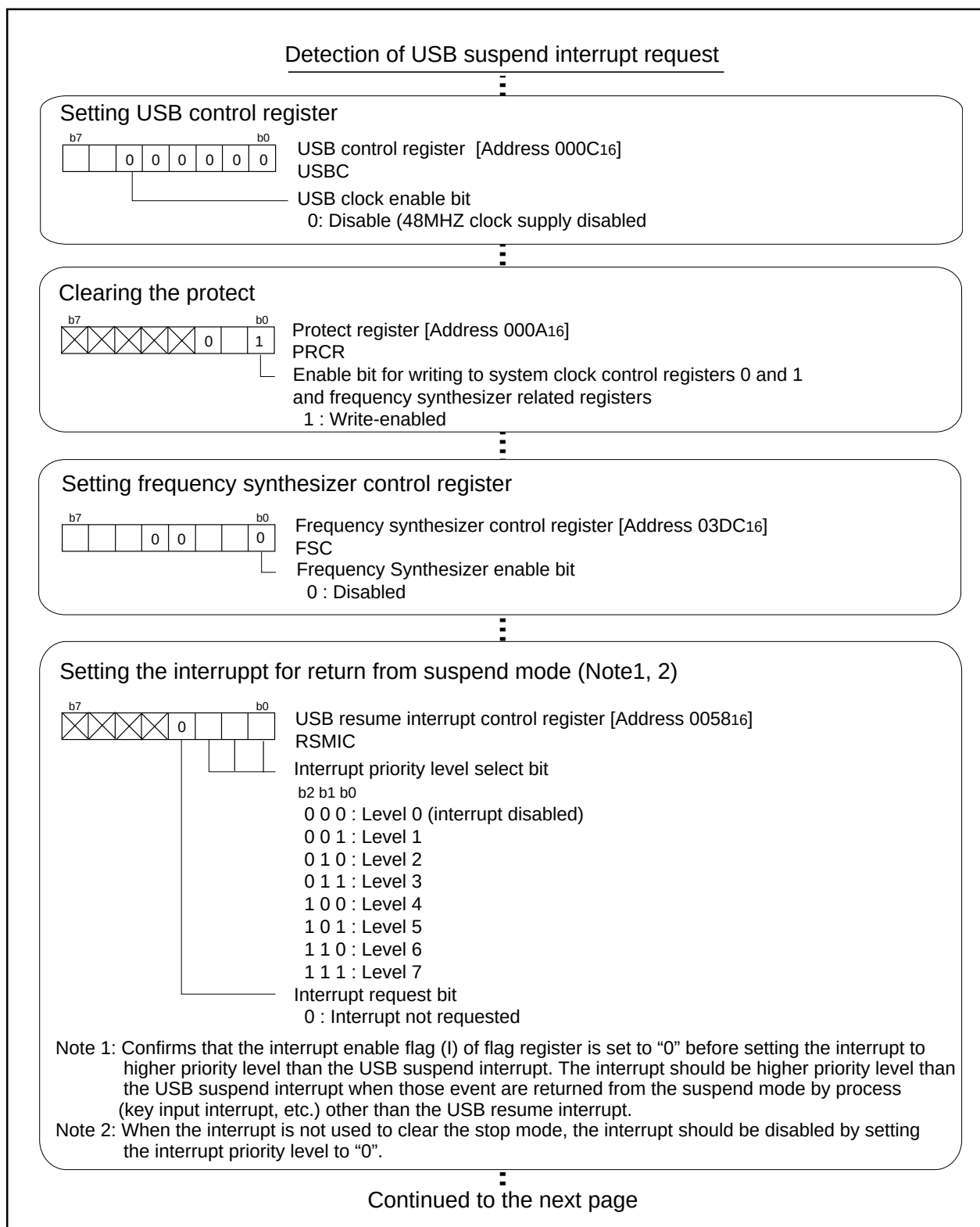
Figure 2.8.28. USB suspend interrupt request processing routine (1)
