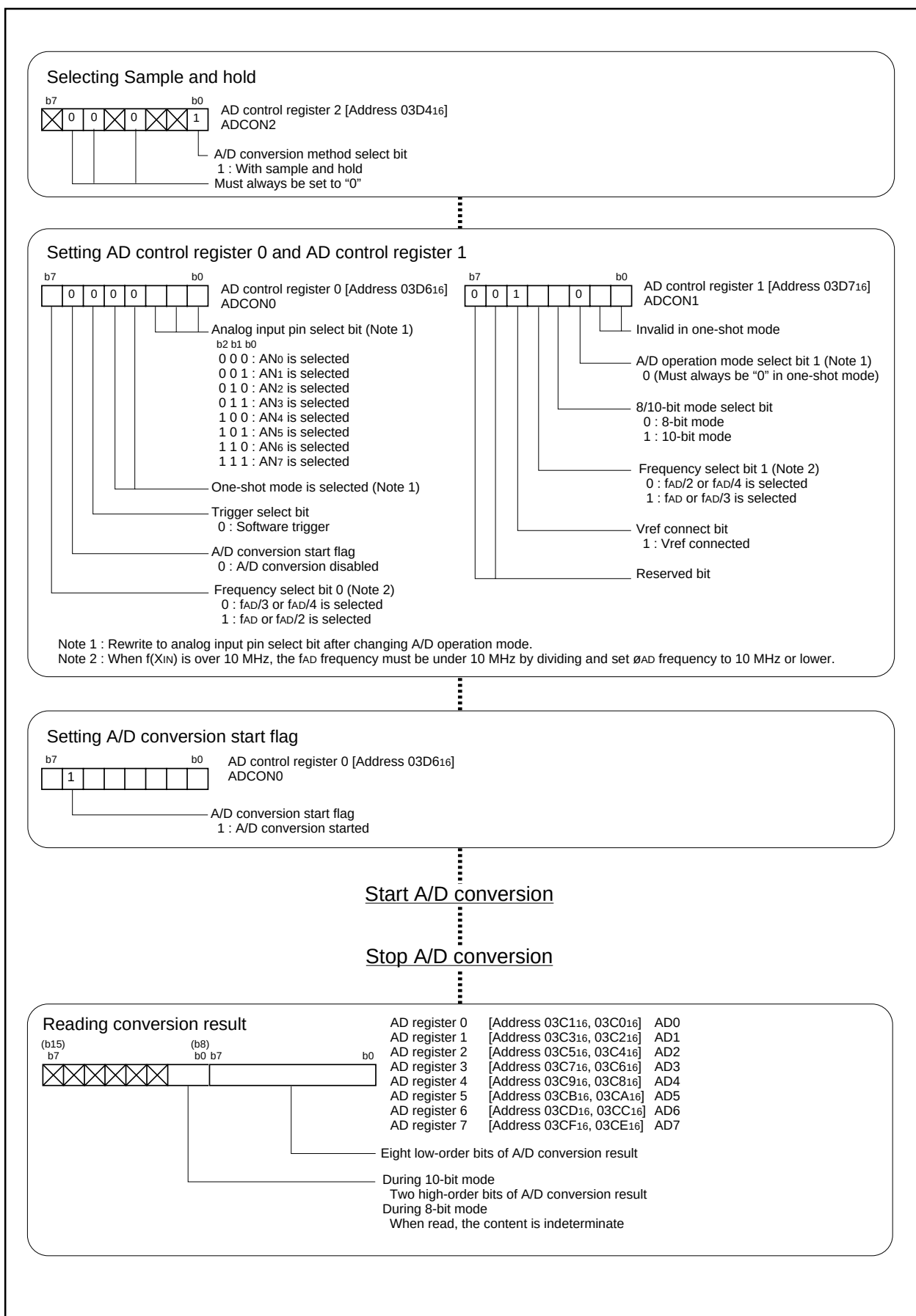
Figure 2.9.5. Set-up procedure of one-shot mode
