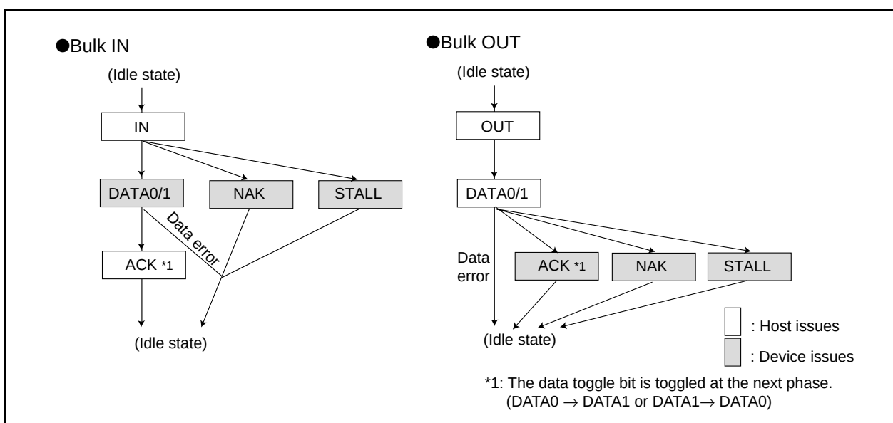
Figure 2.8.5. Bulk transfer
