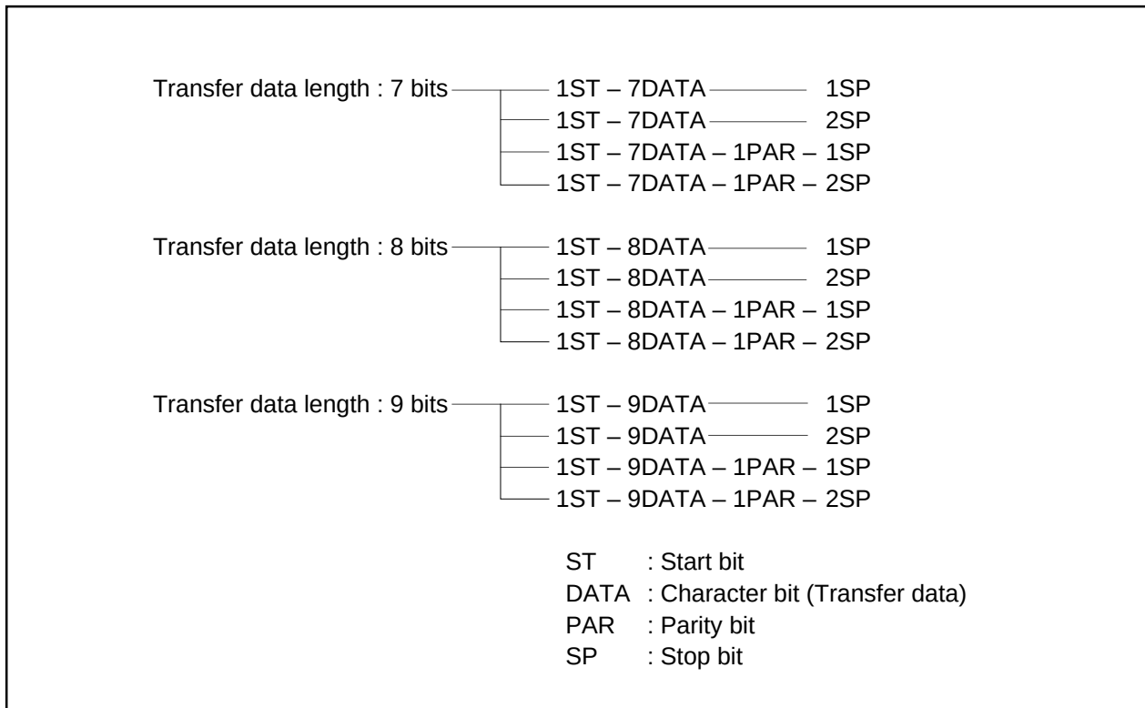
Figure 2.4.1. Transmission/reception format
