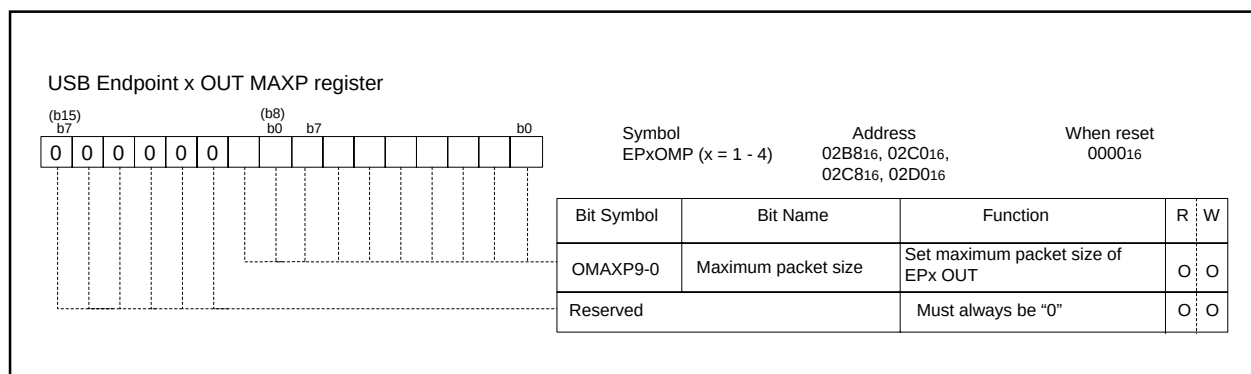
Figure 2.8.41. USB endpoint x(x=1 to 4) OUT MAXP register
