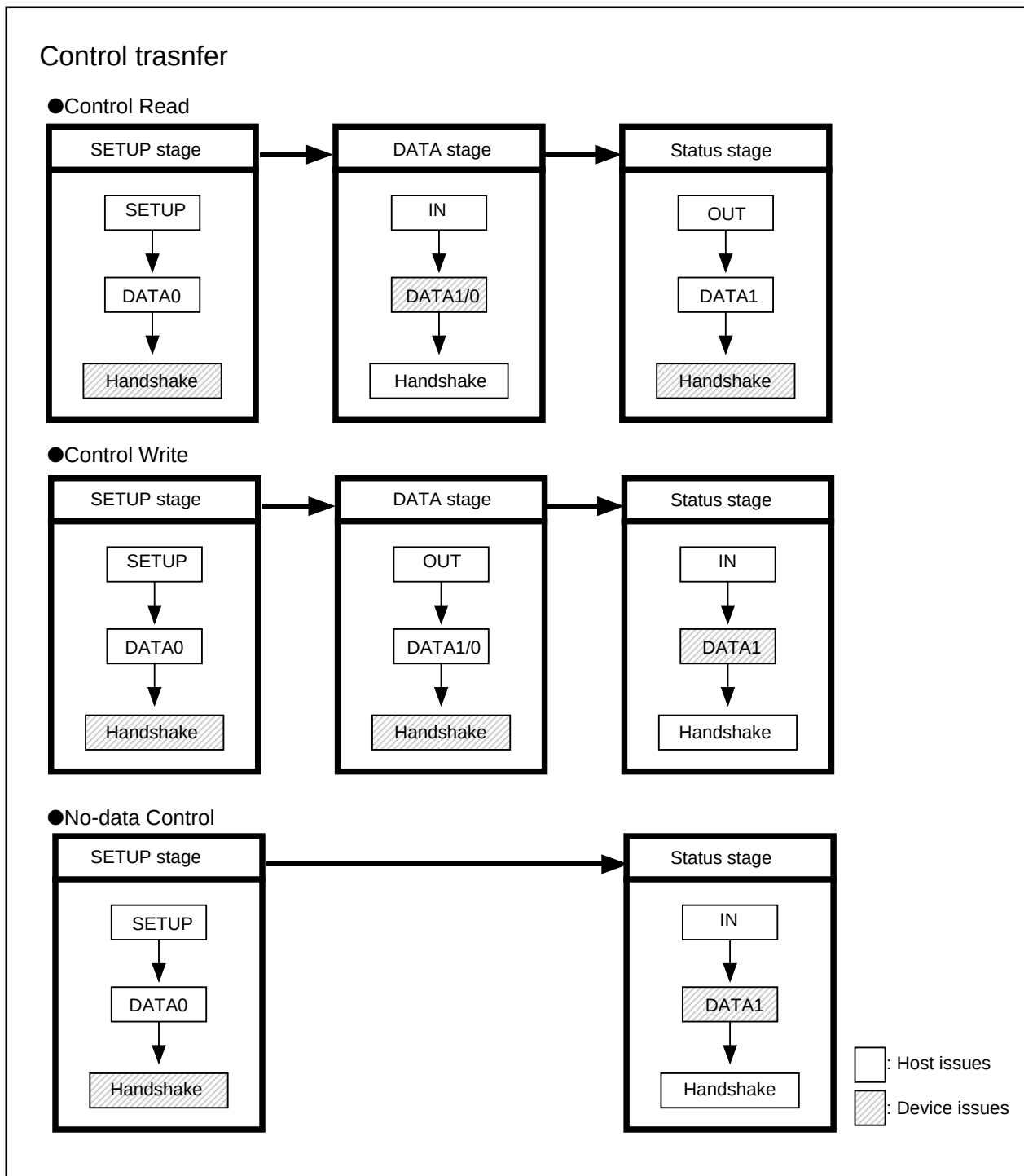
Figure 2.8.4. Control transfer communication sequence
