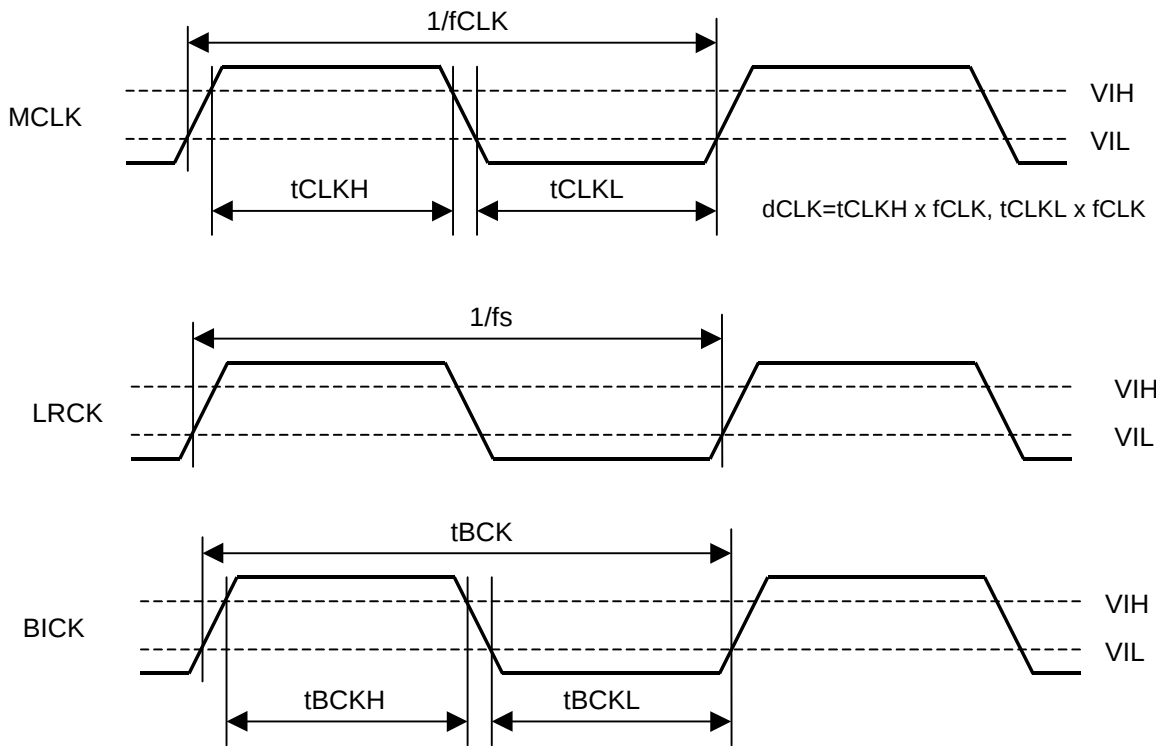
Figure 3. Clock Timing
