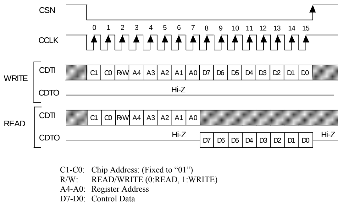
Figure 20. 4-wire Serial Control I/F Timing
