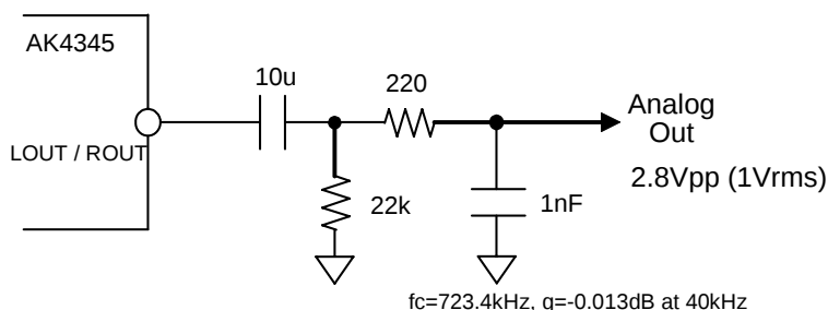
Figure 24. External 1 st order LPF Circuit Example
