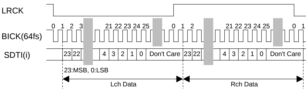
Figure 13. Mode 3 Timing
