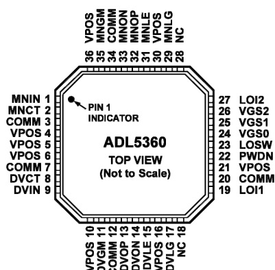
Figure 2. Pin Configuration
