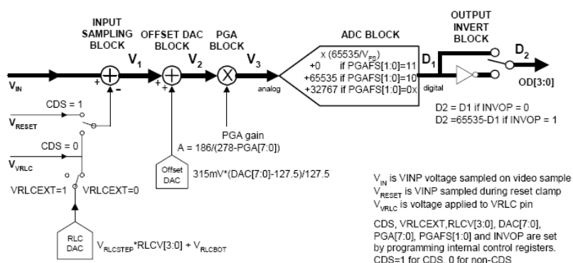
Overall Signal Flow
