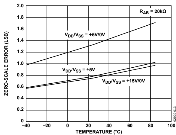
Figure 15. Zero-Scale Error
