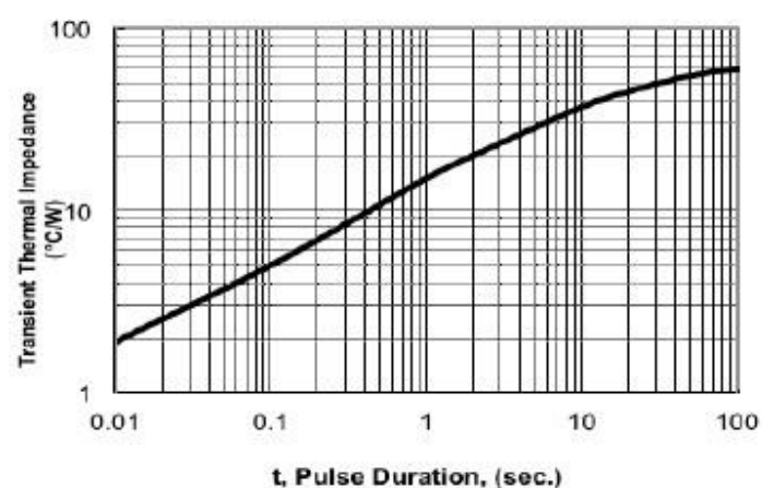
Figure 6. Typical Transient Thermal Impedance
