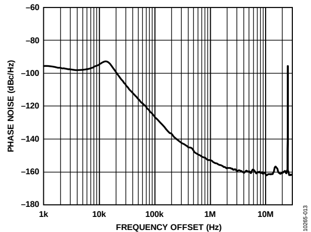
Figure 13. Fractional-N Phase Noise and Spur Performance; Low Spur Mode; V_{CO_{OUT}} = 905.2 MHz, REF_{IN} = 100 MHz, PFD = 25 MHz, Loop Filter Bandwidth = 20 kHz, Channel Spacing = 200 kHz, FRAC = 26, MOD = 125
