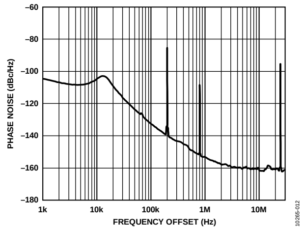
Figure 12. Fractional-N Phase Noise and Spur Performance; Low Noise Mode; V_{CO_{OUT}} = 905.2 MHz, REF_{IN} = 100 MHz, PFD = 25 MHz, Loop Filter Bandwidth = 20 kHz, Channel Spacing = 200 kHz, FRAC = 26, MOD = 125
