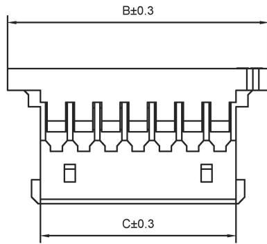
04P~30P Double Salient Scale 1:1
