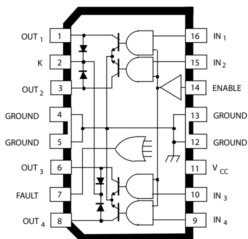
A2557xLB (SOIC)
