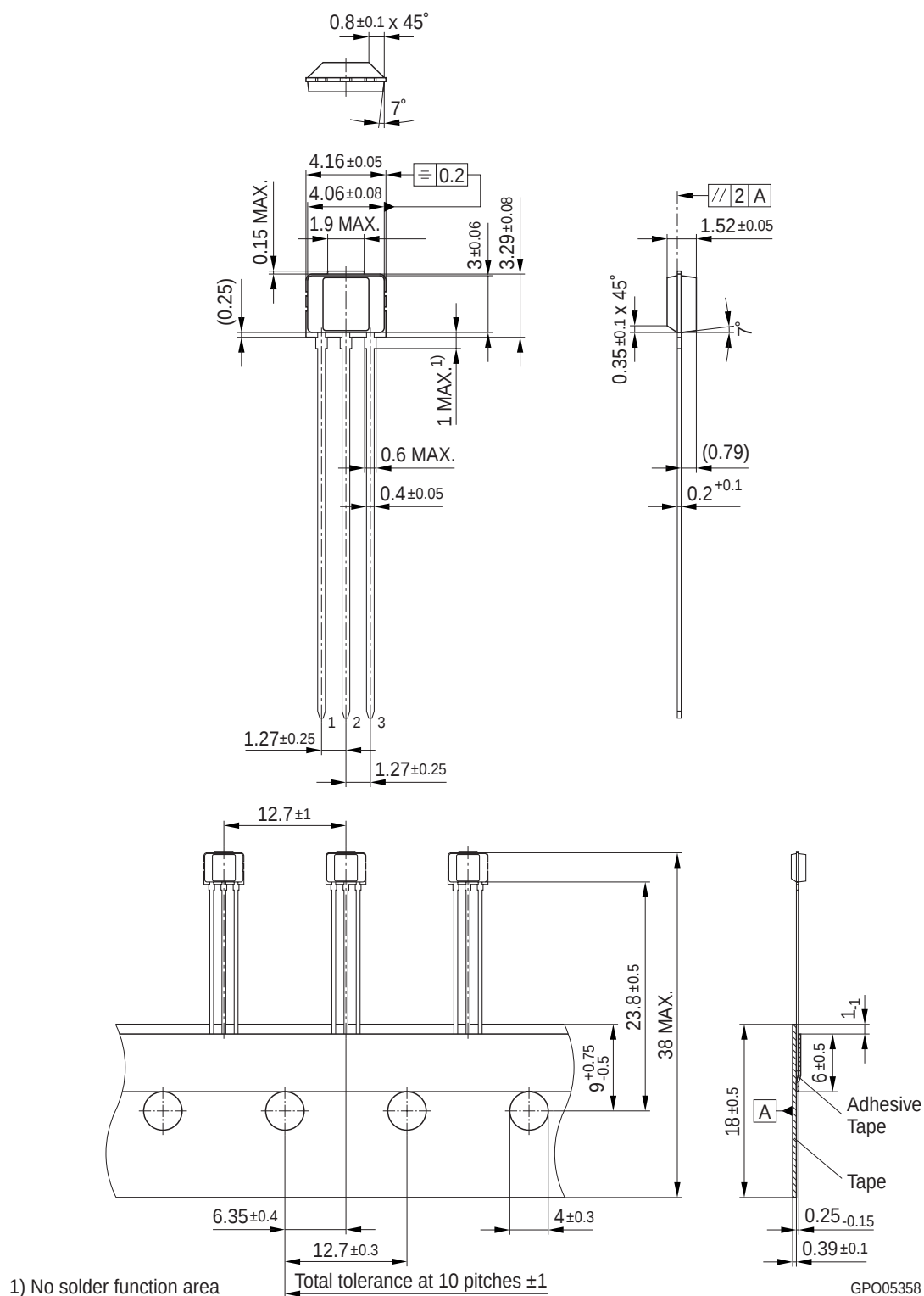
Figure 7 Package outline
