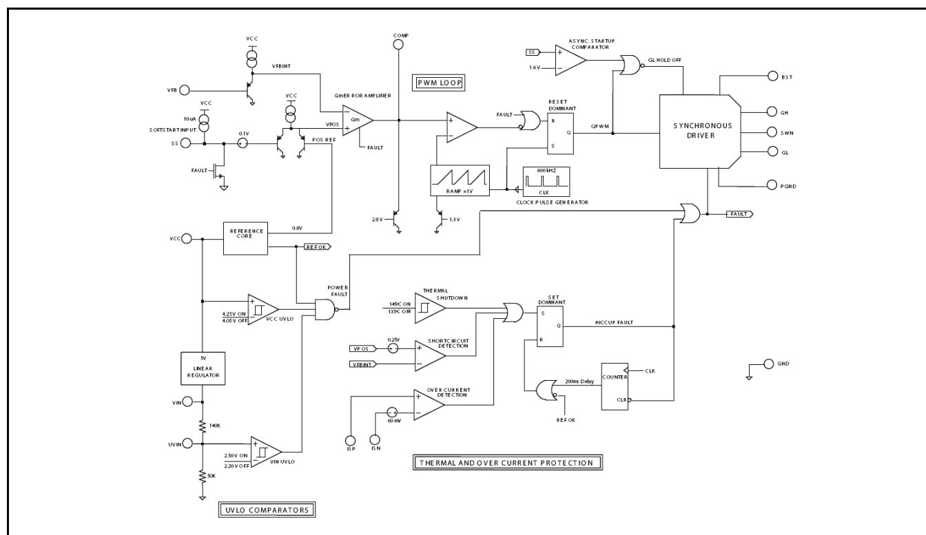
Fig. 2: SP7663 Block Diagram (Exar's 600KHz Controller based)
