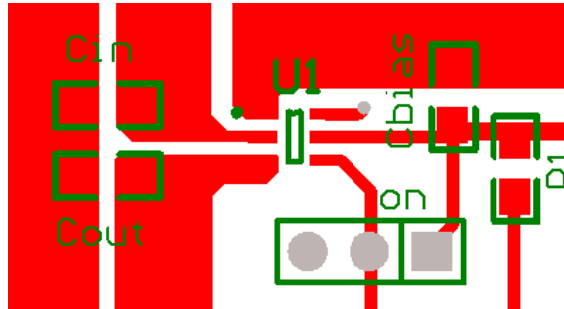
Fig.18 Reference layout
