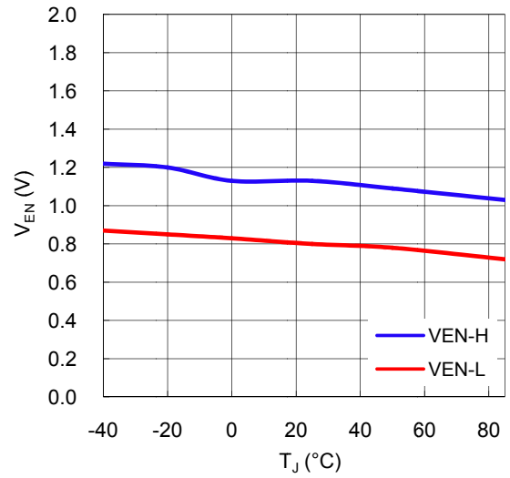
Fig.14 EN Threshold vs. Temperature
