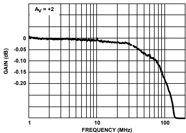
FIGURE 15. GAIN FLATNESS
