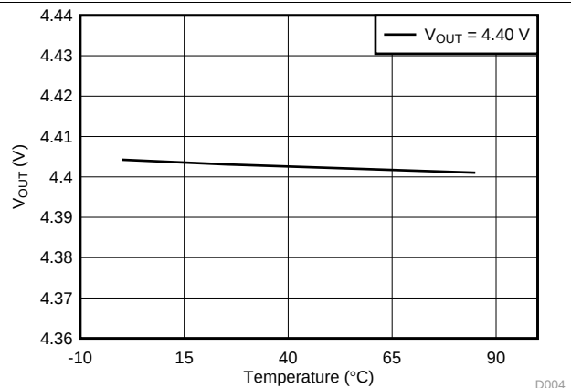
Figure 4. VOUT ADC vs Temperature at 4.4 V
