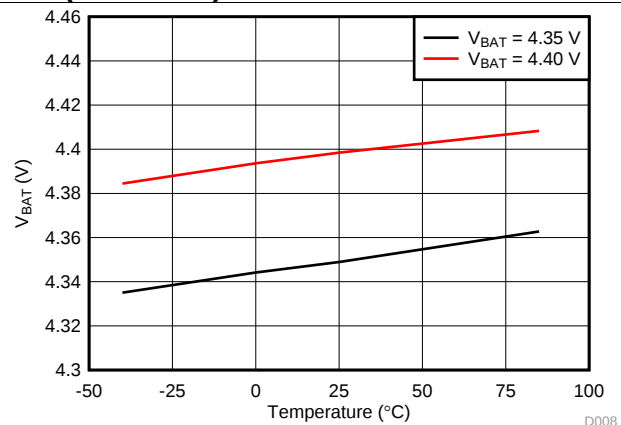
Figure 8. V BAT Regulation vs Temperature
