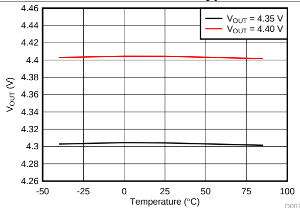
Figure 7. V OUT Regulation vs Temperature
