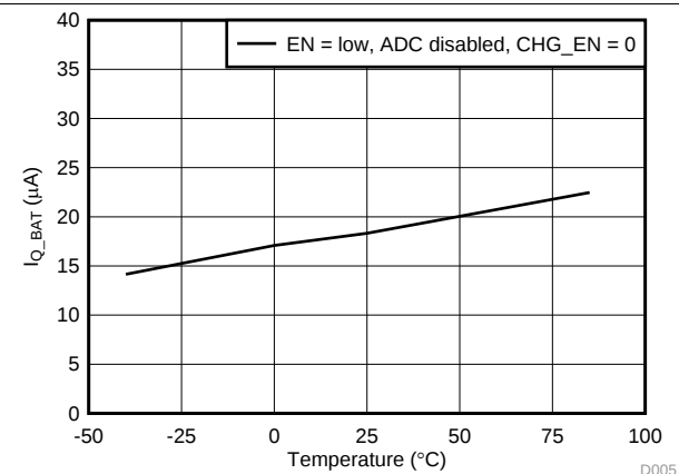
Figure 5. Quiescent Current with Battery Only vs Temperature
