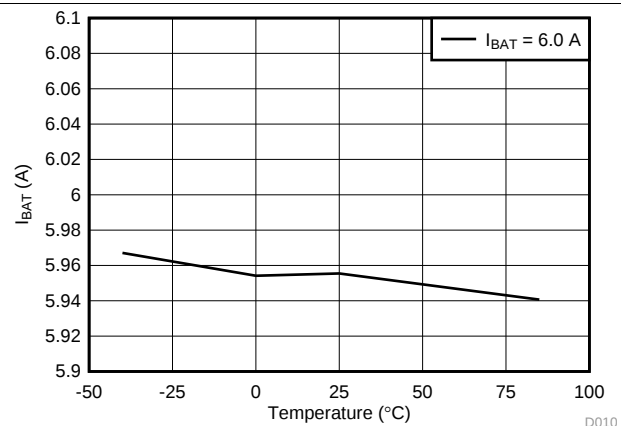
Figure 10. I BAT Regulation vs Temperature at 6 A
