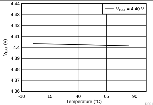
Figure 1. VBAT ADC vs Temperature at 4.4 V
