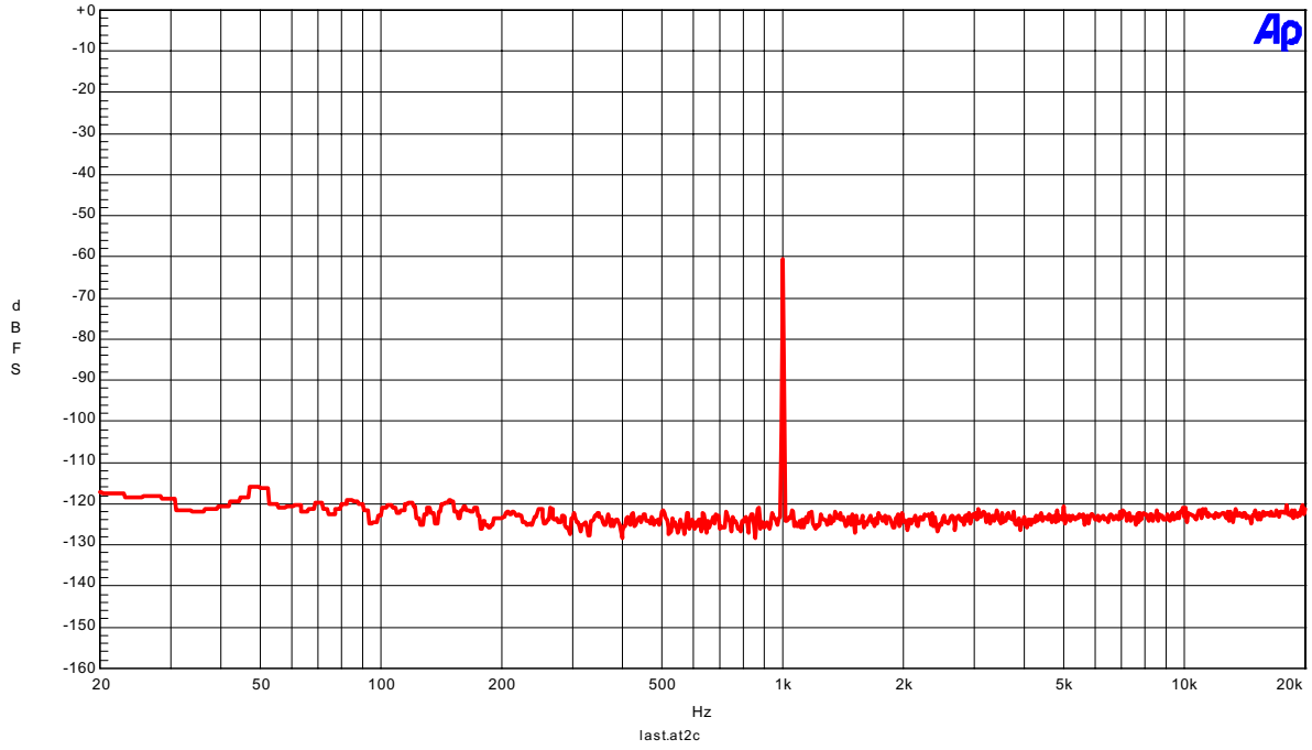
Figure 7. FFT Plot
