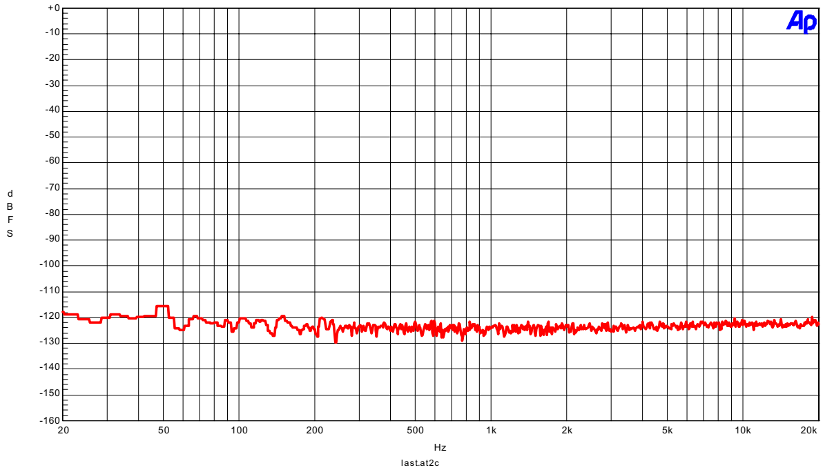
Figure 8. FFT Plot
