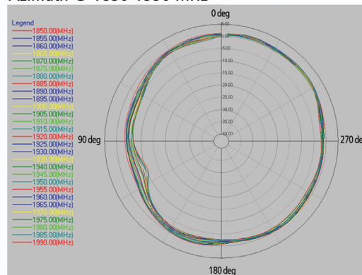
Azimuth @ 1850-1990 MHz
