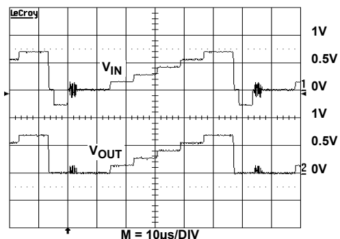
FIGURE 30. VIDEO SIGNAL
