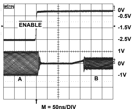
FIGURE 32. ENABLE SIGNAL
