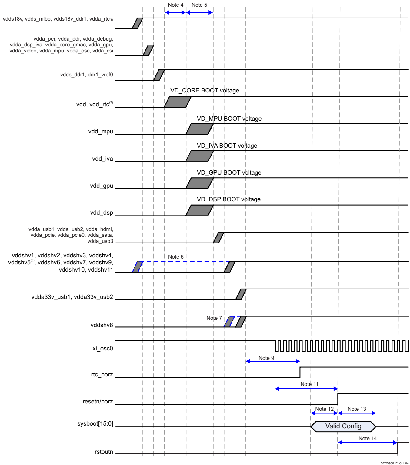
Figure 5-4. Power-Up Sequencing
