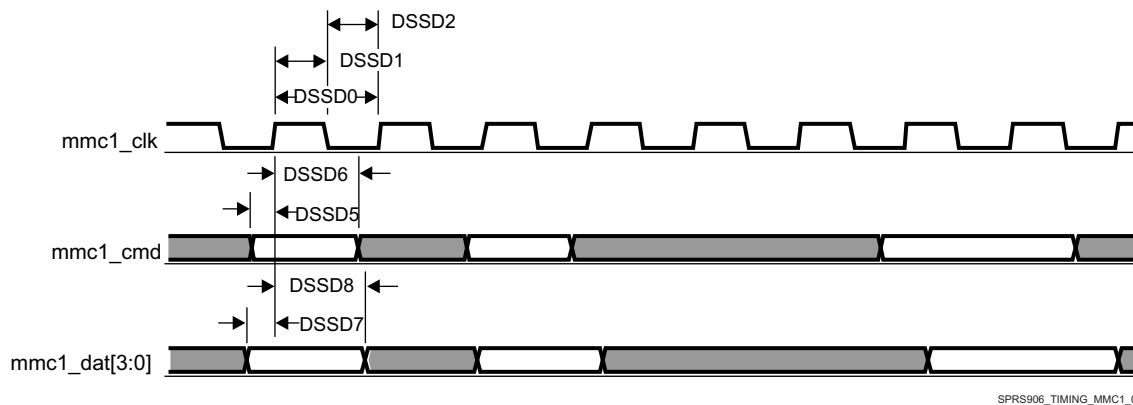
Figure 7-63. MMC/SD/SDIO in - Default Speed - Receiver Mode
