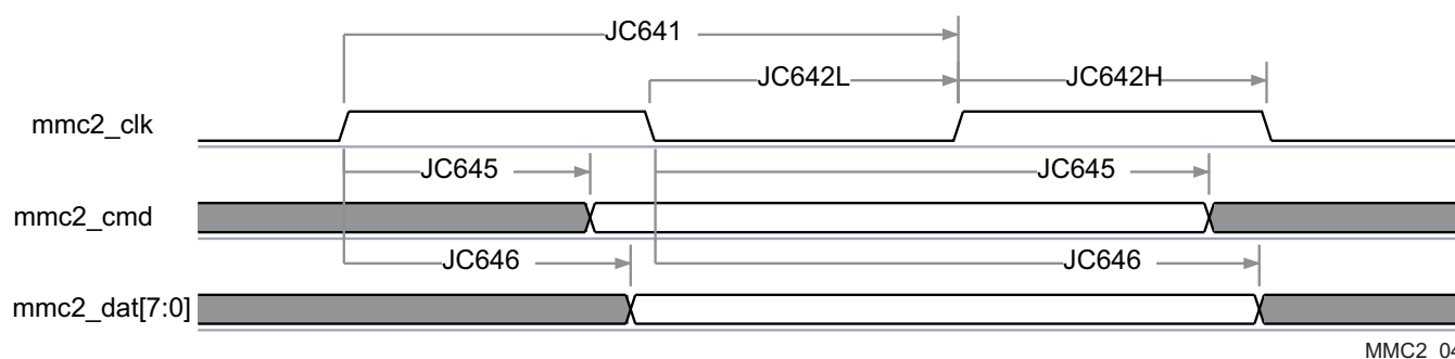
Figure 7-80. MMC/SD/SDIO in - High Speed JC64 - transmitter Mode
