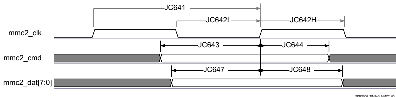
Figure 7-79. MMC/SD/SDIO in - High Speed JC64 - Receiver Mode
