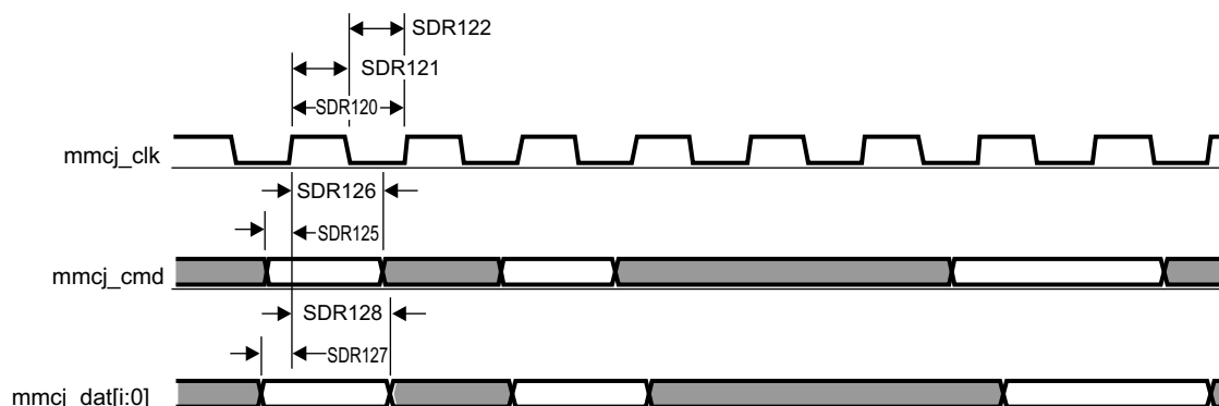
Figure 7-88. MMC/SD/SDIOj in - SDR12 - Receiver Mode
