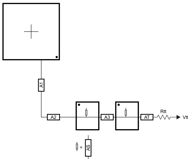
Figure 8-54. ADDR_CTRL Routing for Two Single-Side DDR3 Devices
