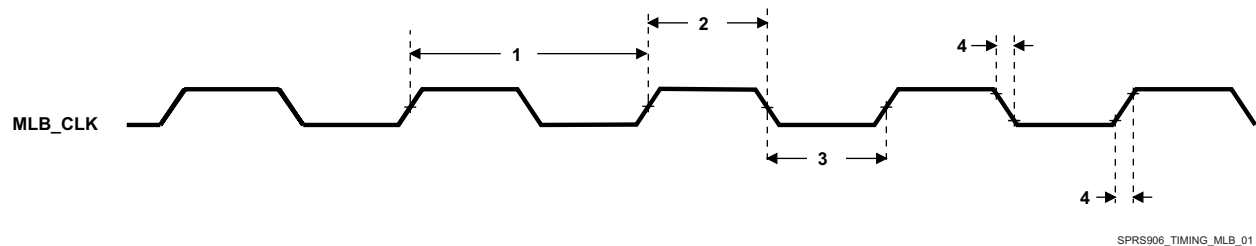
Figure 7-62. MLB_CLK Timing
