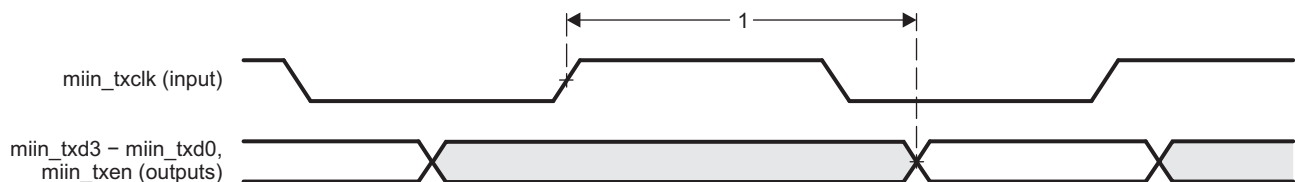
Figure 7-56. GMAC Transmit Interface Timing MII operation
