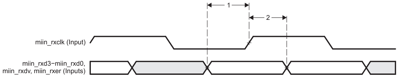
Figure 7-55. GMAC Receive Interface Timing MII operation
