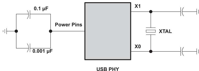
Figure 8-25. Power Supply and Clock Connection to the USB PHY
