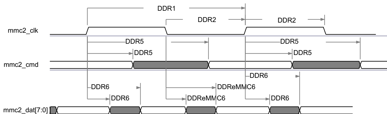
Figure 7-83. MMC/SD/SDIO in - High Speed DDR JC64 - Transmitter Mode
