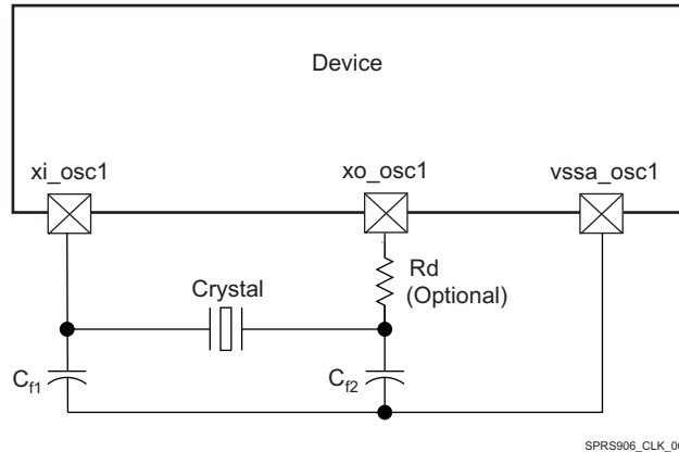
Figure 6-6. Crystal Implementation
