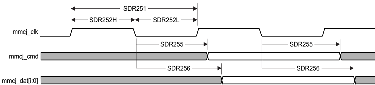
Figure 7-91. MMC/SD/SDIOj in - SDR25 - Transmitter Mode
