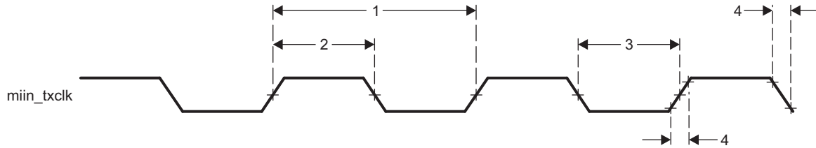
Figure 7-54. Clock Timing (GMAC Transmit) - MII operation
