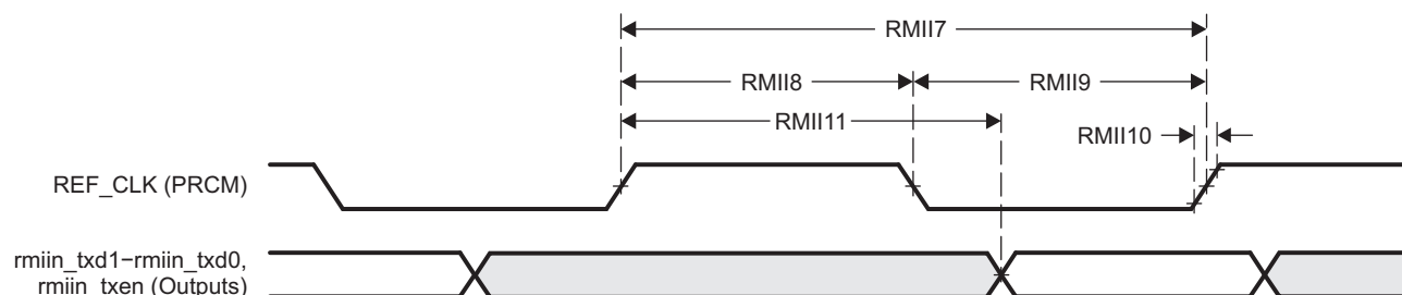
Figure 7-59. GMAC Transmit Interface Timing RMII n Operation
