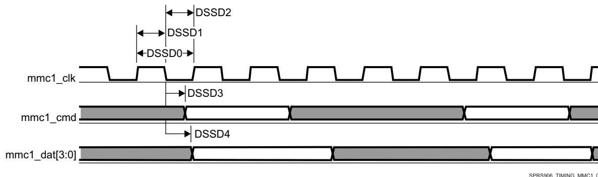
Figure 7-64. MMC/SD/SDIO in - Default Speed - Transmitter Mode
