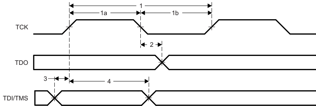
Figure 7-95. JTAG Timing
