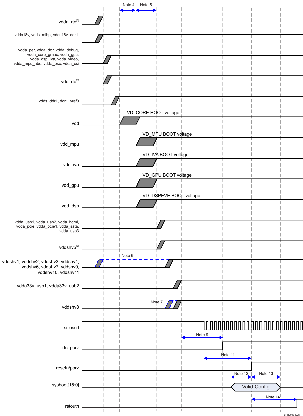
Figure 5-1. Power-Up Sequencing
