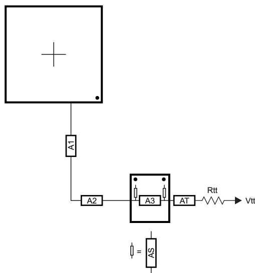
Figure 8-56. ADDR_CTRL Routing for Two Mirrored DDR3 Devices
