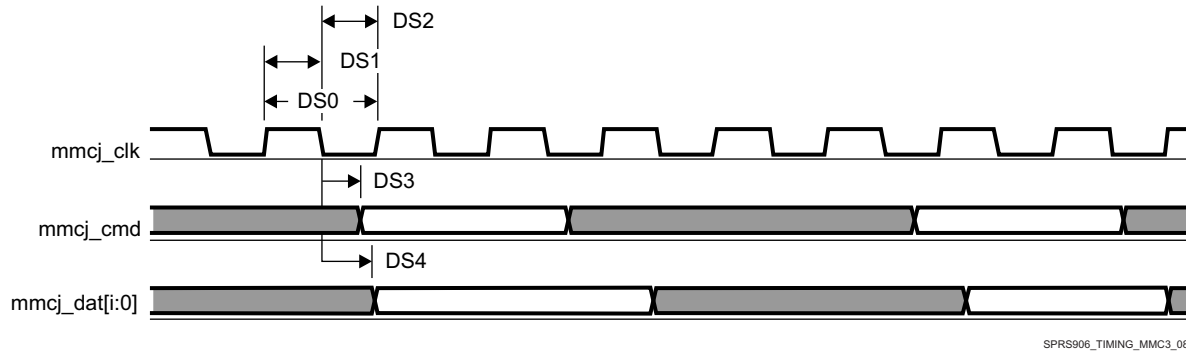
Figure 7-85. MMC/SD/SDIOj in - Default Speed - Transmitter Mode
