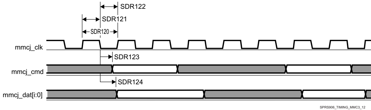
Figure 7-89. MMC/SD/SDIOj in - SDR12 - Transmitter Mode
