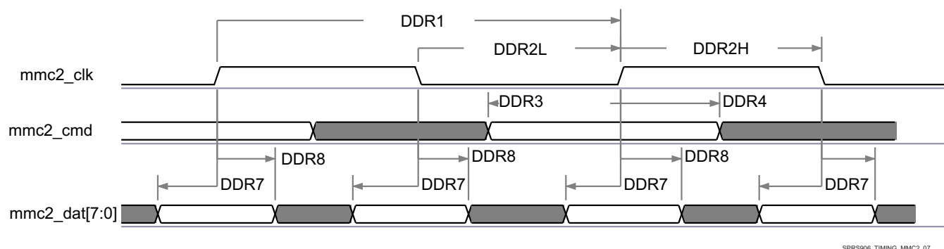
Figure 7-82. MMC/SD/SDIO in - High Speed DDR JC64 - Receiver Mode
