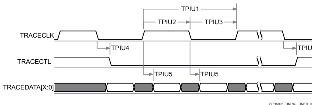
Figure 7-97. TPIU-PLL DDR Transmit Mode (1)
