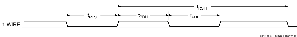
Figure 7-29. 1-Wire-Break (Reset)
