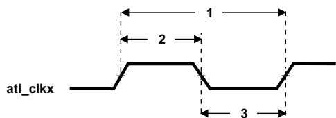
Figure 7-94. ATL_CLKOUTx Timing
