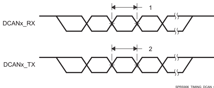
Figure 7-52. DCANx Timings
