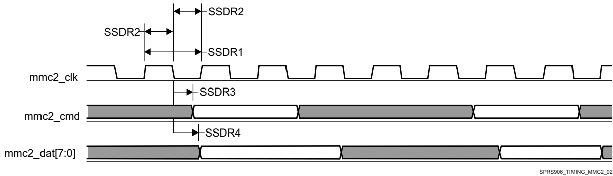
Figure 7-78. MMC/SD/SDIO in - Standard JC64 - Transmitter Mode
