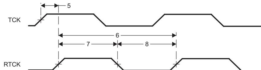
Figure 7-96. JTAG With RTCK Timing
