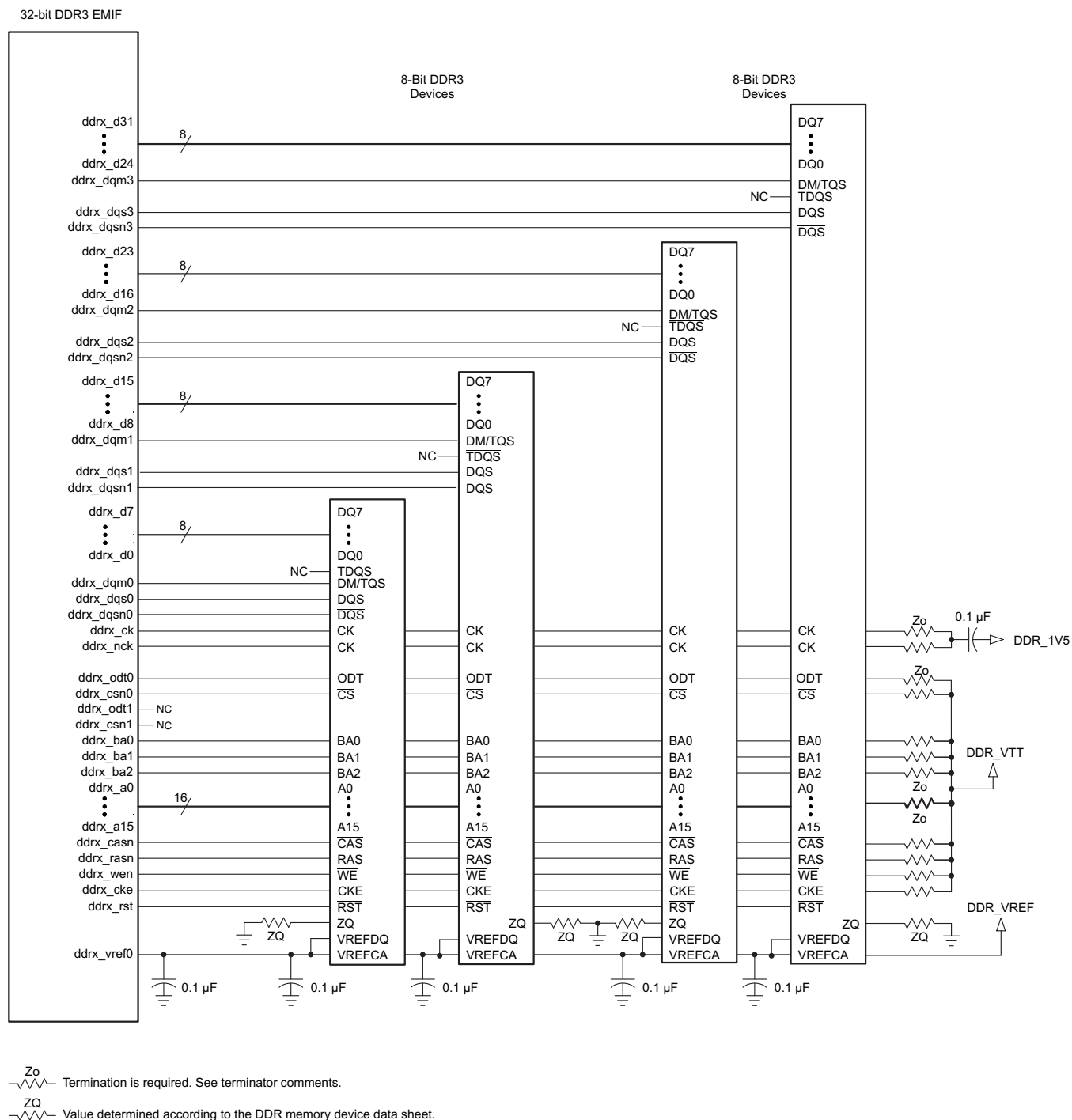
Figure 8-42. 32-Bit, One-Bank DDR3 Interface Schematic Using Four 8-Bit DDR3 Devices
