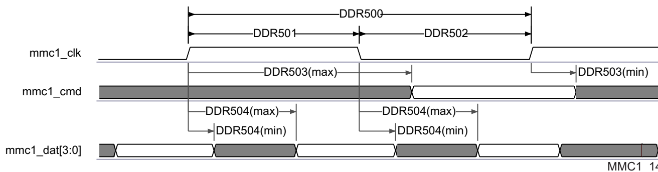
Figure 7-76. SDMMC - High Speed SD - DDR - Data/Command Transmit
