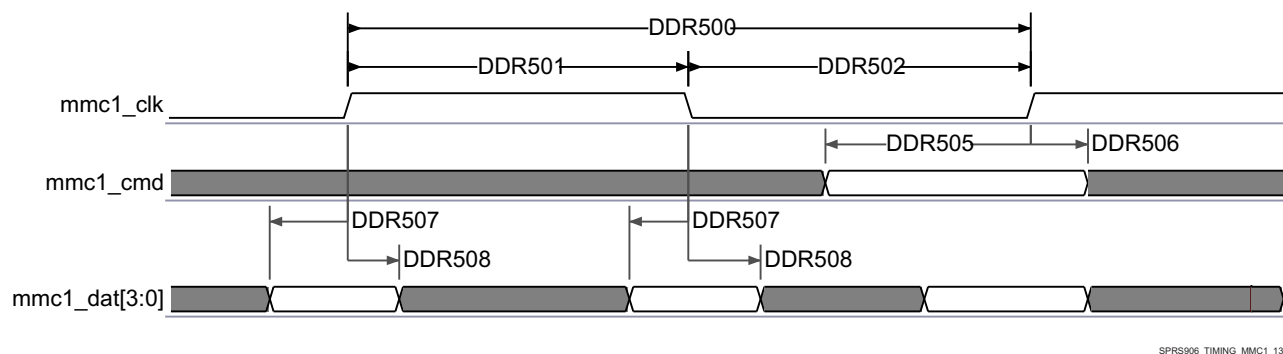
Figure 7-75. SDMMC - High Speed SD - DDR - Data/Command Receive
