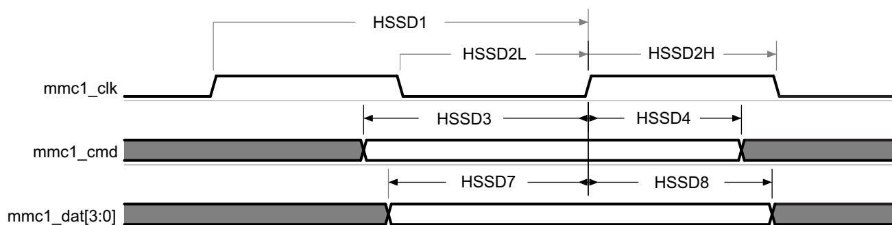
Figure 7-65. MMC/SD/SDIO in - High Speed - Receiver Mode
