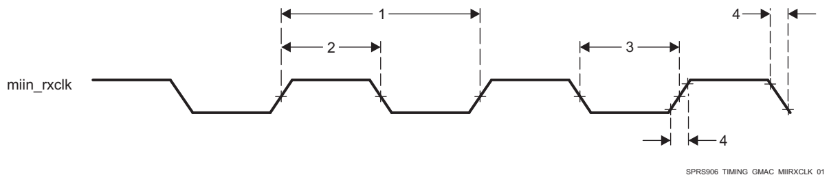
Figure 7-53. Clock Timing (GMAC Receive) - MIIn operation
