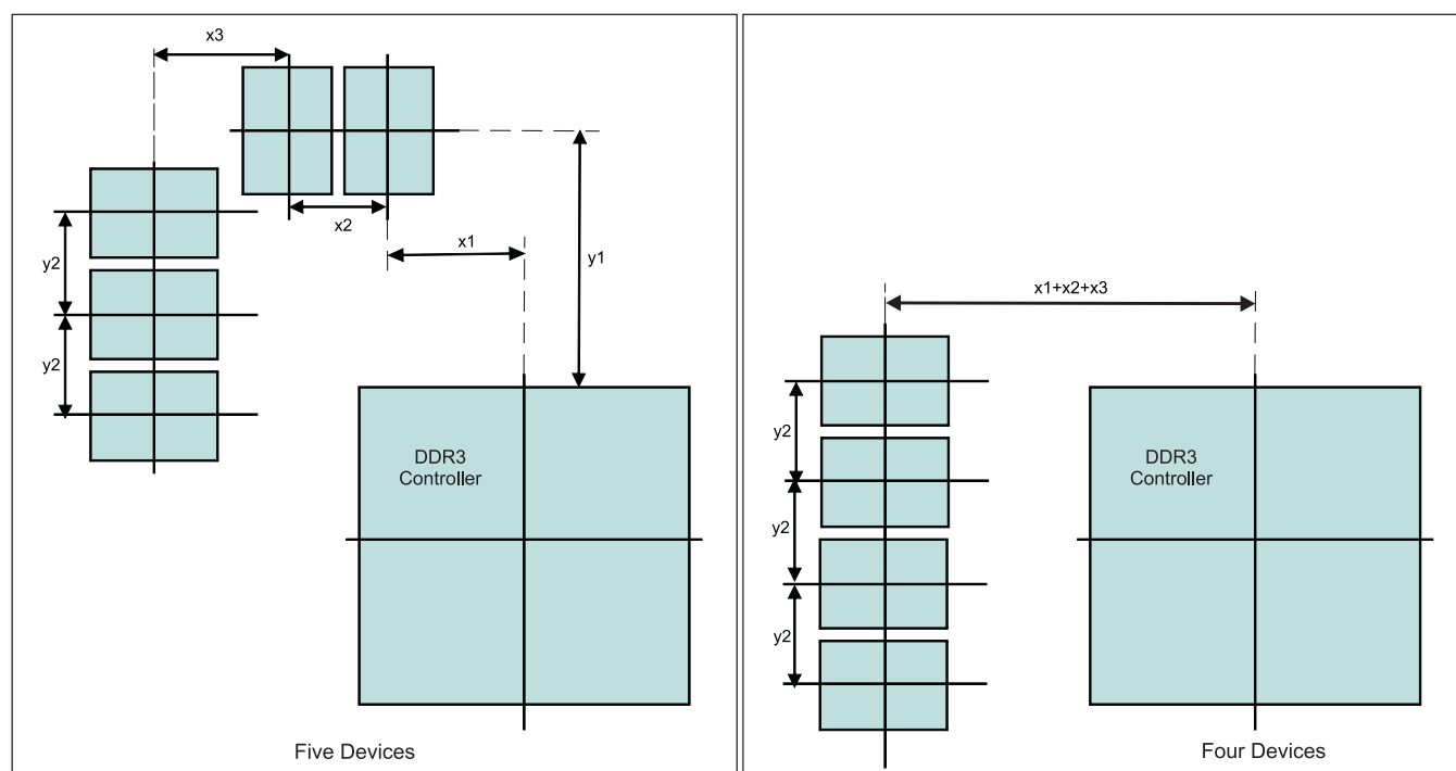
Figure 8-43. Placement Specifications
