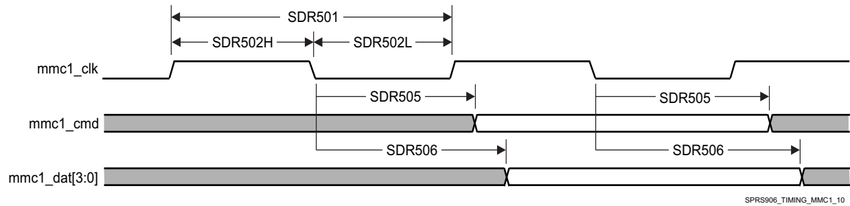
Figure 7-72. MMC/SD/SDIO in - High Speed SDR50 - Transmitter Mode
