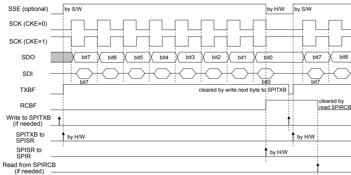
FIGURE 2.10: SPI Mode Timing (Master Mode)
