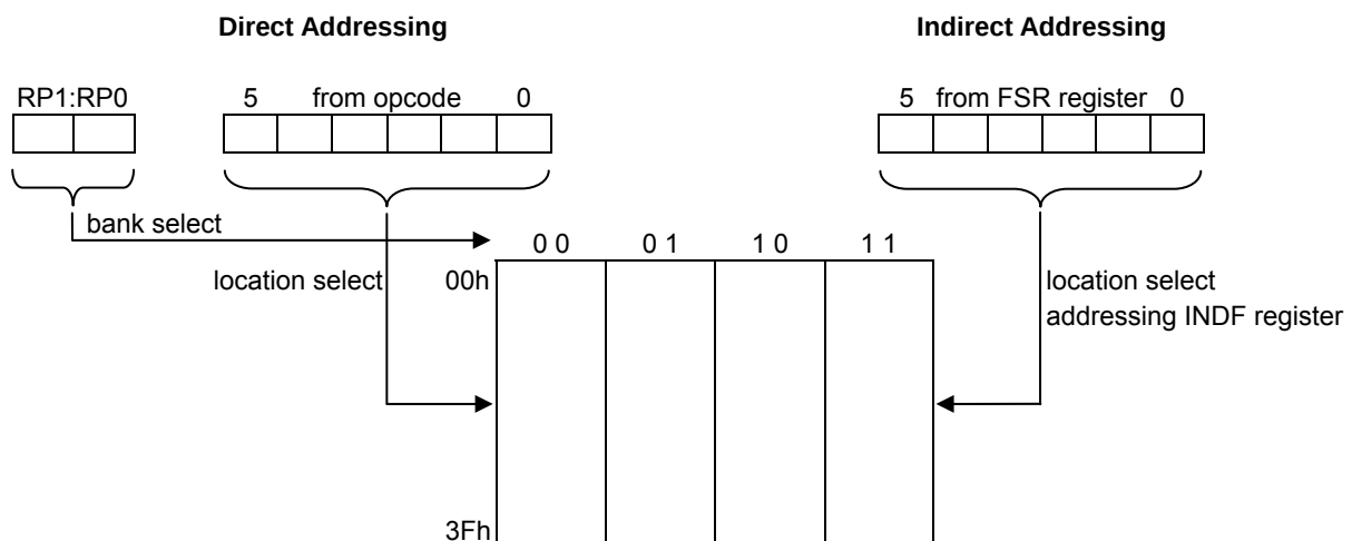
FIGURE 2.1: Direct/Indirect Addressing for FM8PE51 Series
