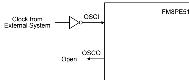
FIGURE 2.18: HF, or LF Oscillator Modes (External Clock Input Operation)
