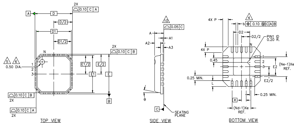
Figure 5-1. QFN24 Package Information
