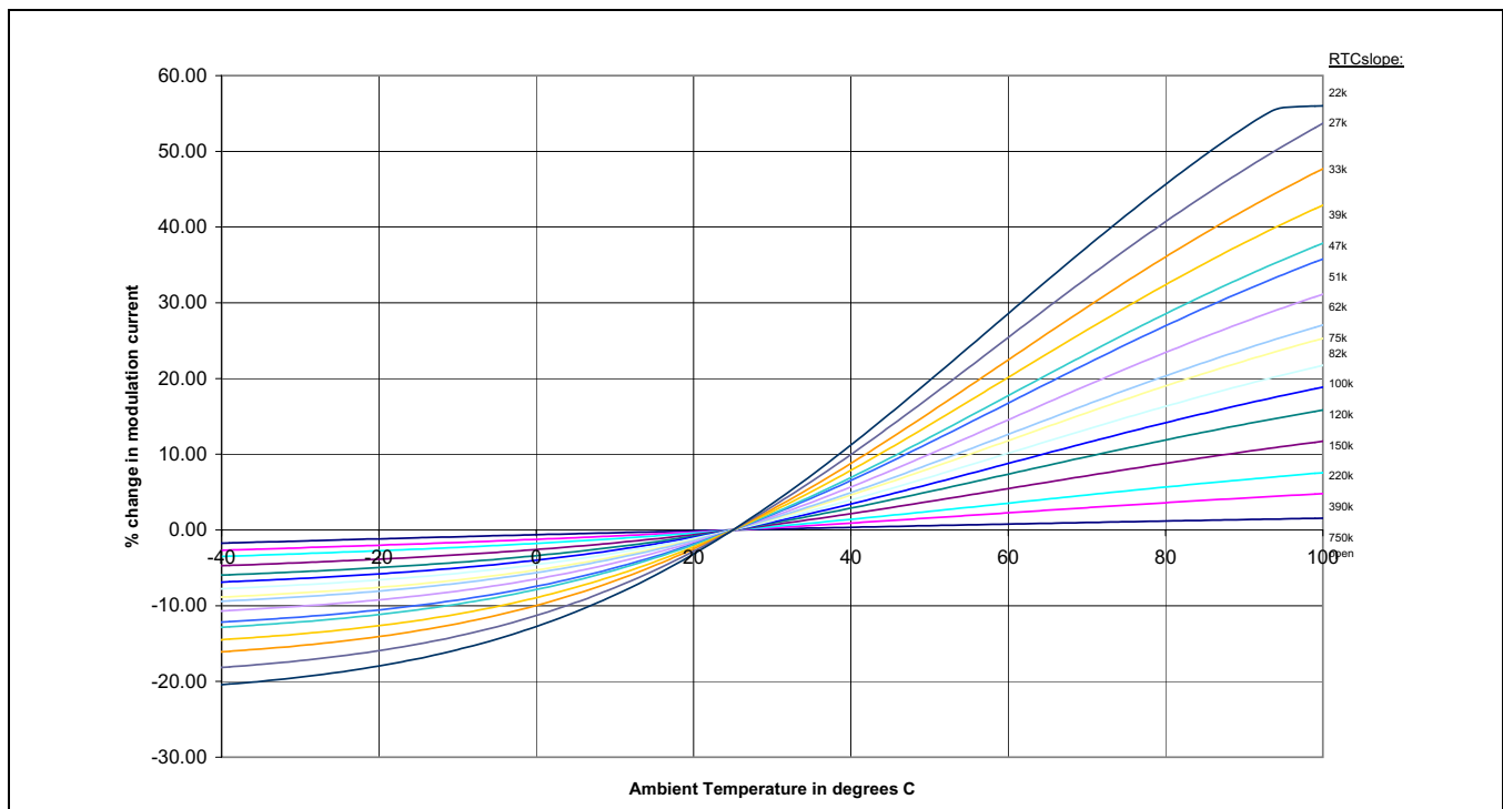
Figure 3-2. Selecting TC SLOPE resistance in common anode configuration
